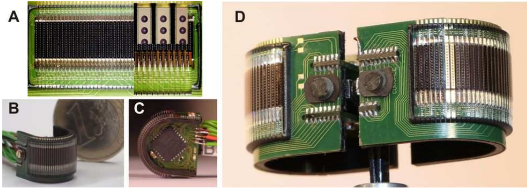
Figure 1.10: CurvACE ommatidia and prototype assembly. (A) Image of the planar ommatidial array just after assembly and column dicing. (Right Inset) Details of the microlens array surface, as well as the wire bonding between the photoreceptor and the interconnection layers, are shown. Perspective image of the CurvACE prototype (B), top view (C), and configured to provide a 360° field of view (FOV).
