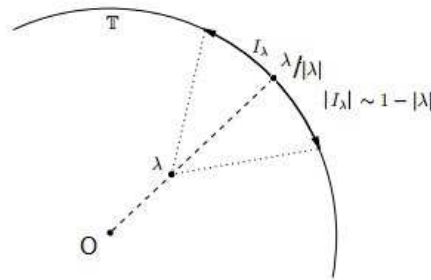
FIGURE 3.1 – Privalov shadow.
