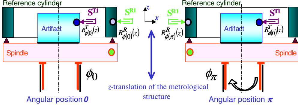
Figure 11. Schematic description of the modified reversal separation method. S^{T1} and S^{R1} represent the designations of respectively measuring part probe and reference probe. To perform this technique, two straightness measurements should be carried out. The first straightness measurement must be carried out for angular position 0 and the two probes must be in the same corner and direction. The second measurement must be carried out for angular position \pi . For this configuration, both the reference probe and reference cylinder are shifted by the angle of \pi . The direction of the two probes becomes opposite. To perform this method, the metrological structure should ensure two degrees of freedom ( z -translation and z -rotation). The z -rotation of the metrological structure can cause additional positioning errors and this solution should be avoided.
