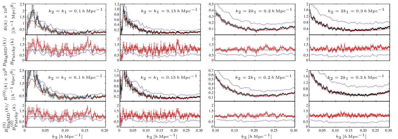
Figure 3. Halo bispectrum for the BIGMD N -body simulations and PATCHY mock catalogues as a function of k_3 . Top panels show the bispectrum in real space and bottom panels the bispectrum monopole in redshift space. Different columns present different scales and shapes as labelled. Same colour notation that in Fig. 2 is used.
