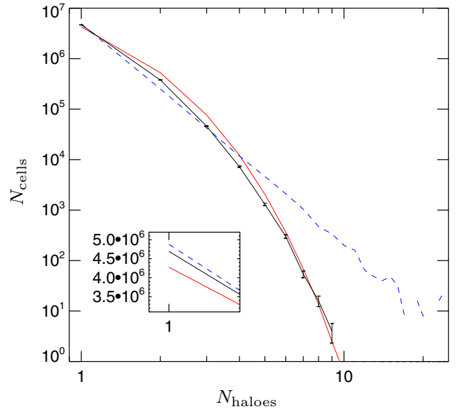
Figure 1. Halo PDF showing the number of cells N_{\text{cells}} hosting the same number of haloes N_{\text{haloes}} with a cell resolution of (2.5 h^{-1} \text{ Mpc})^3 . In red PATCHY (with \rho_{\text{th}}^{\text{High}} ) and in black BIGMD including the error bars extracted from the PATCHY mock catalogues. In addition, one PATCHY mock catalogue in dashed blue (with \rho_{\text{th}}^{\text{Low}} ) ignoring the shape of the halo PDF. The latter has been multiplied by eight to compensate for the eight times smaller volume, and hence, about eight times smaller number of haloes. The number density (which determines the integral of the PDF) is the same in all catalogues (see equation 7). The inset shows the first bin of the halo PDF for cells containing only one halo.
