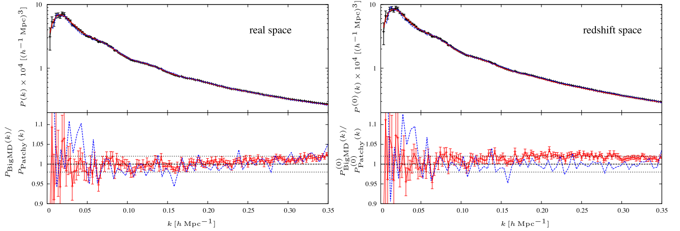
Figure 2. Halo power spectrum for BIGMD N -body simulation (black symbols in the top sub-panels) and for PATCHY mock catalogues (red lines with \rho_{\text{th}}^{\text{High}} and dashed blue lines with \rho_{\text{th}}^{\text{Low}} ). The left-hand panel shows real space power spectrum and the right-hand panel the redshift space monopole power spectrum. The power spectrum for the PATCHY mock catalogues with \rho_{\text{th}}^{\text{High}} corresponds to the average over 20 independent realizations. Only the errors corresponding to the BIGMD N -body simulations are shown for clarity. In the bottom sub-panels, the relative deviation between BIGMD and PATCHY is shown. Black dotted lines indicate 2 per cent deviation.
