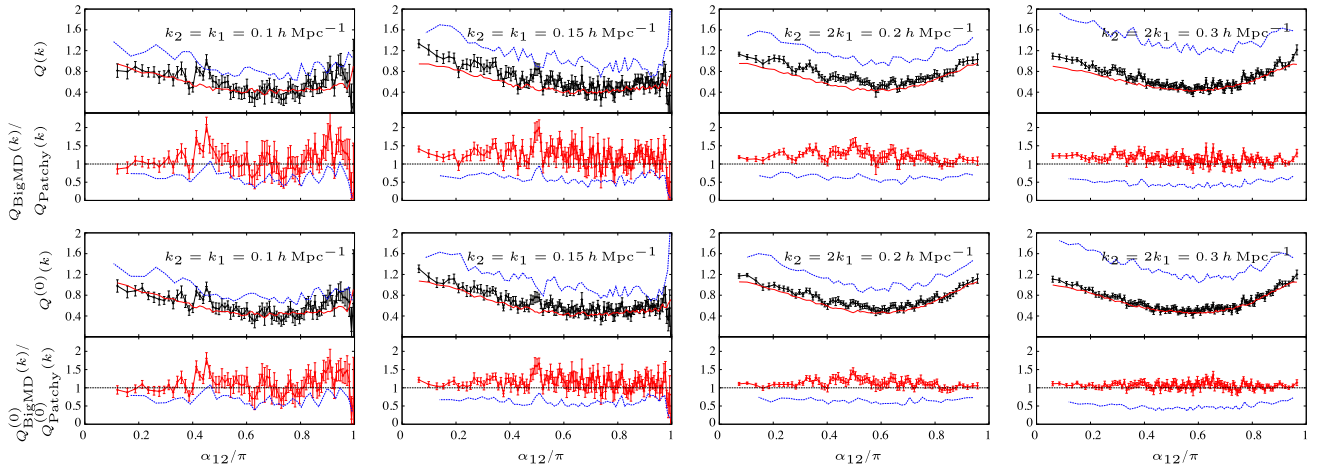
Figure 4. Halo reduced bispectrum for BiGMD N -body simulations and PATCHY mock catalogues as a function of the angle between k_1 and k_2 , \alpha_{12} . Same colour and panel notation that in Fig. 3 is used.
