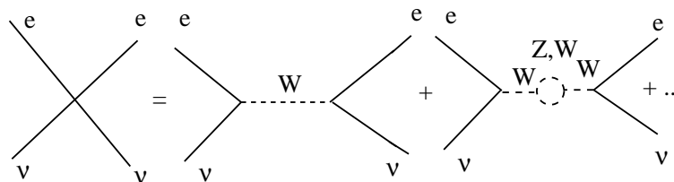
Fig. 3 The 4 Fermi interaction is the sum over all ‘virtual’ W and Z boson exchanges. At low energy mainly the ‘tree’ graph contributes.
