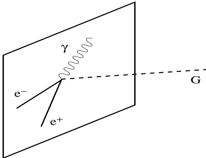
Fig. 4 The confinement of matter to the brane, while gravity propagates in the bulk (from [43]).
