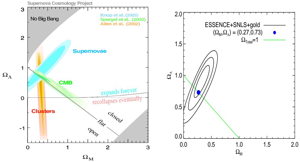
Fig. 1 Observational constraints in the (\Omega_m, \Omega_\Lambda) plane: joint constraints (left) (from [8]); recent compilation of supernova constraints (right) (from [9]). The line \Omega_K = \Omega_m + \Omega_\Lambda - 1 = 0 is also indicated.
