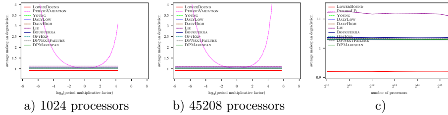
Figure 54: Evaluation of the different heuristics on a Petascale platform with Exponential failures ( MTBF = 125 years), using Numerical Kernel law with \gamma = 1 , and variable overhead model ( C(p) = 600 \frac{45208}{p} )
