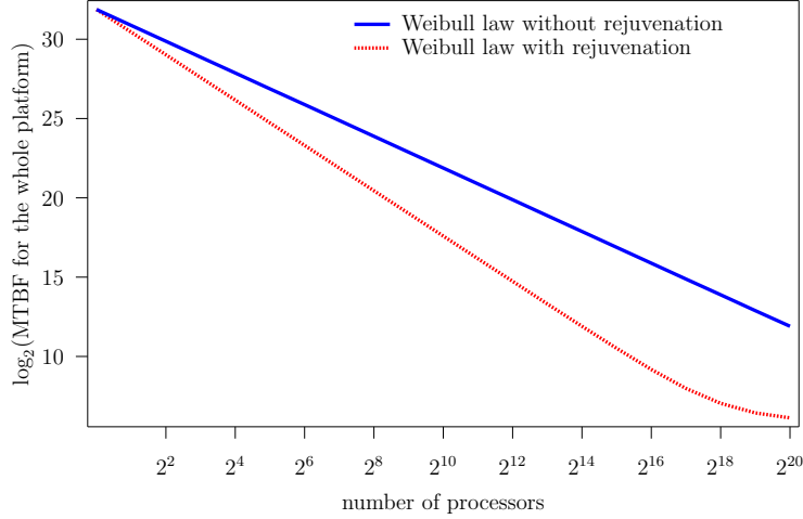
Figure 1: Impact of the two rejuvenation options on the platform MTBF for a Weibull distribution with shape parameter 0.70, a processor-level MTBF of 125 years, and a downtime of 60 seconds.
