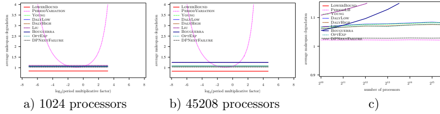
Figure 75: Evaluation of the different heuristics on a Petascale platform with Weibull failures ( MTBF = 125 years), using Amdahl law with \gamma = 10^{-6} , and variable overhead model ( C(p) = 600 \frac{45208}{p} )
