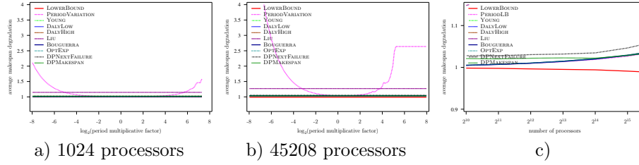
Figure 17: Evaluation of the different heuristics on a Petascale platform with Exponential failures ( MTBF = 500 years), using Numerical Kernel law with \gamma = 0.1 , and constant overhead model
