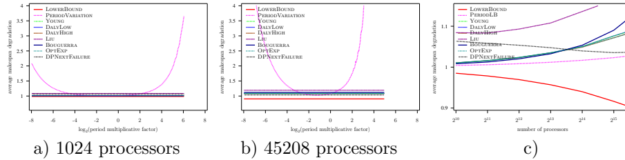
Figure 59: Evaluation of the different heuristics on a Petascale platform with Weibull failures ( MTBF = 500 years), using embarrassingly parallel job, and constant overhead model
