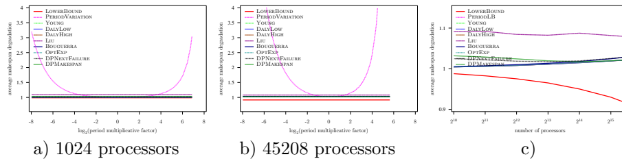
Figure 20: Evaluation of the different heuristics on a Petascale platform with Exponential failures ( MTBF = 125 years), using Numerical Kernel law with \gamma = 10 , and constant overhead model
