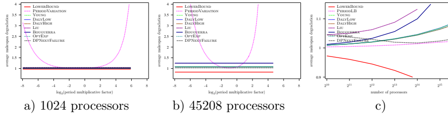
Figure 64: Evaluation of the different heuristics on a Petascale platform with Weibull failures ( MTBF = 125 years), using Numerical Kernel law with \gamma = 0.1 , and constant overhead model
