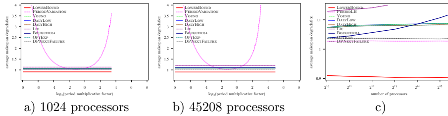
Figure 72: Evaluation of the different heuristics on a Petascale platform with Weibull failures ( MTBF = 500 years), using embarrassingly parallel job, and variable overhead model ( C(p) = 600 \frac{45208}{p} )
