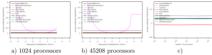
Figure 31: Evaluation of the different heuristics on a Petascale platform with Exponential failures ( MTBF = 500 years), using Numerical Kernel law with \gamma = 1 , and variable overhead model ( C(p) = 600 \frac{45208}{p} )
