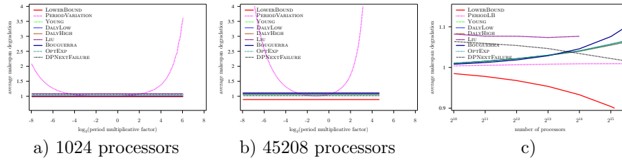
Figure 61: Evaluation of the different heuristics on a Petascale platform with Weibull failures ( MTBF = 500 years), using Amdahl law with \gamma = 10^{-4} , and constant overhead model
