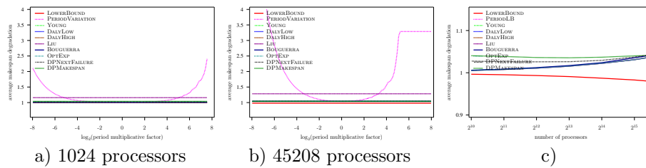
Figure 41: Evaluation of the different heuristics on a Petascale platform with Exponential failures ( MTBF = 500 years), using Numerical Kernel law with \gamma = 0.1 , and constant overhead model
