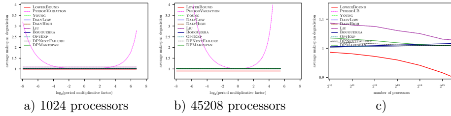
Figure 36: Evaluation of the different heuristics on a Petascale platform with Exponential failures ( MTBF = 125 years) using Amdahl law with \gamma = 10^{-4} , and constant overhead model
