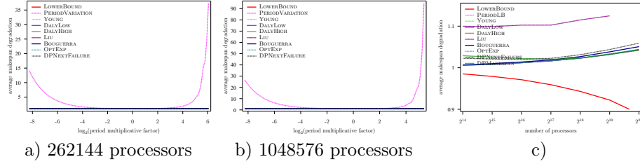
Figure 86: Evaluation of the different heuristics on a Exascale platform with Exponential failures ( MTBF = 1250 years), using Numerical Kernel law with \gamma = 1 , and constant overhead model
