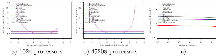
Figure 33: Evaluation of the different heuristics on a Petascale platform with Exponential failures ( MTBF = 500 years), using Numerical Kernel law with \gamma = 10 , and variable overhead model ( C(p) = 600 \frac{45208}{p} )
