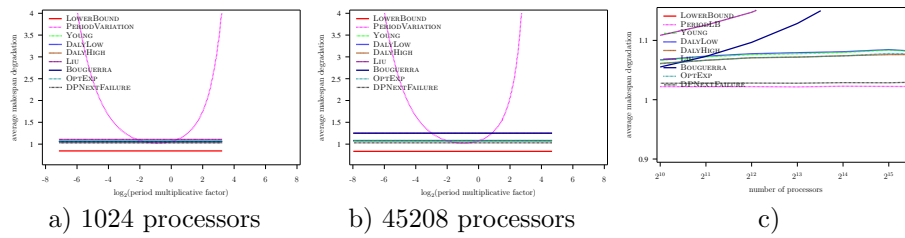
Figure 77: Evaluation of the different heuristics on a Petascale platform with Weibull failures ( MTBF = 125 years), using Numerical Kernel law with \gamma = 0.1 , and variable overhead model ( C(p) = 600 \frac{45208}{p} )
