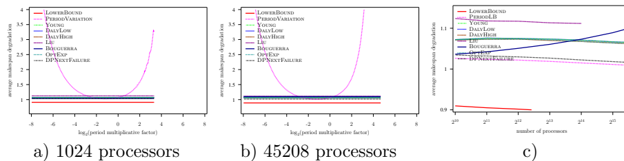
Figure 74: Evaluation of the different heuristics on a Petascale platform with Weibull failures ( MTBF = 500 years), using Amdahl law with \gamma = 10^{-4} , and variable overhead model ( C(p) = 600 \frac{45208}{p} )
