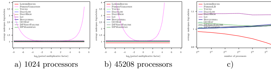
Figure 44: Evaluation of the different heuristics on a Petascale platform with Exponential failures ( MTBF = 125 years), using Numerical Kernel law with \gamma = 10 , and constant overhead model
