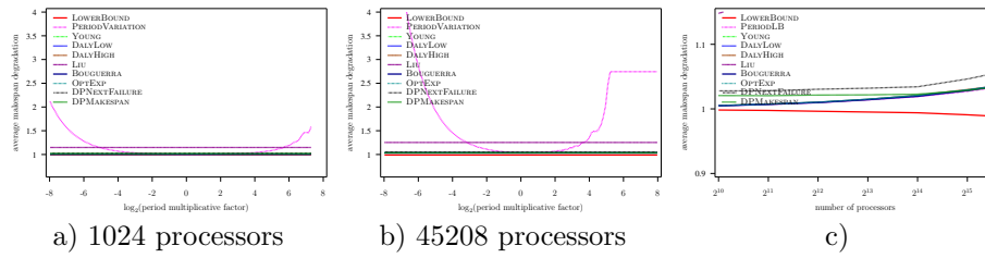
Figure 15: Evaluation of the different heuristics on a Petascale platform with Exponential failures ( MTBF = 500 years), using Amdahl law with \gamma = 10^{-6} , and constant overhead model
