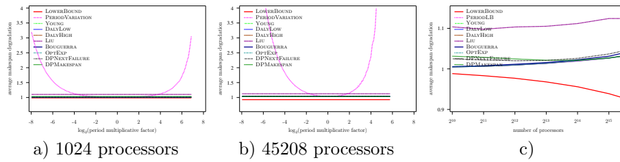
Figure 16: Evaluation of the different heuristics on a Petascale platform with Exponential failures ( MTBF = 125 years), using Numerical Kernel law with \gamma = 0.1 , and constant overhead model
