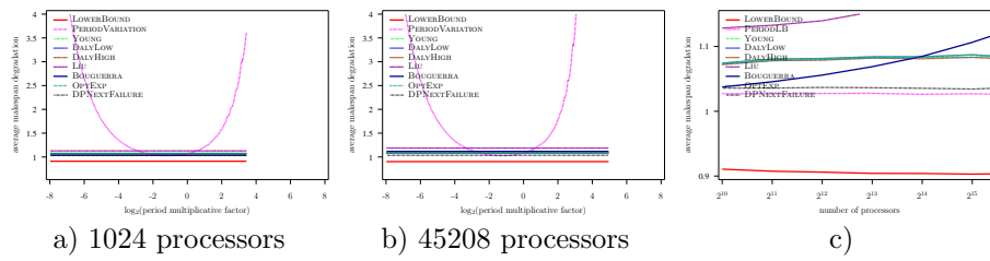
Figure 76: Evaluation of the different heuristics on a Petascale platform with Weibull failures ( MTBF = 500 years), using Amdahl law with \gamma = 10^{-6} , and variable overhead model ( C(p) = 600 \frac{45208}{p} )
