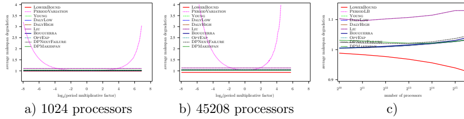
Figure 10: Evaluation of the different heuristics on a Petascale platform with Exponential failures ( MTBF = 125 years) using using embarrassingly parallel job, and constant overhead model
