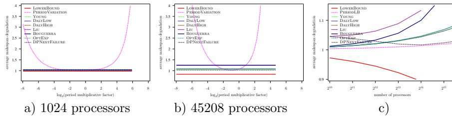
Figure 62: Evaluation of the different heuristics on a Petascale platform with Weibull failures ( MTBF = 125 years), using Amdahl law with \gamma = 10^{-6} , and constant overhead model
