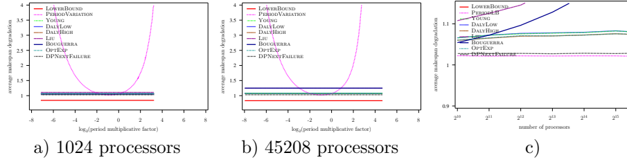
Figure 79: Evaluation of the different heuristics on a Petascale platform with Weibull failures ( MTBF = 125 years), using Numerical Kernel law with \gamma = 1 , and variable overhead model ( C(p) = 600 \frac{45208}{p} )
