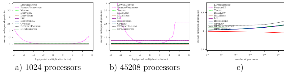
Figure 11: Evaluation of the different heuristics on a Petascale platform with Exponential failures ( MTBF = 500 years) using using embarrassingly parallel job, and constant overhead model
