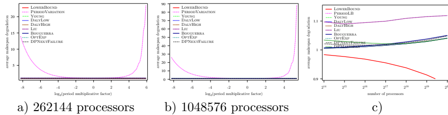
Figure 91: Evaluation of the different heuristics on a Exascale platform with Exponential failures ( MTBF = 1250 years), using Numerical Kernel law with \gamma = 1 , and constant overhead model
