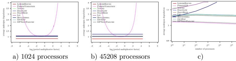
Figure 73: Evaluation of the different heuristics on a Petascale platform with Weibull failures ( MTBF = 125 years), using Amdahl law with \gamma = 10^{-4} , and variable overhead model ( C(p) = 600 \frac{45208}{p} )
