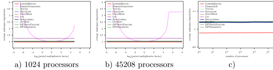
Figure 47: Evaluation of the different heuristics on a Petascale platform with Exponential failures ( MTBF = 500 years), using embarrassingly parallel job, and variable overhead model ( C(p) = 600 \frac{45208}{p} )
