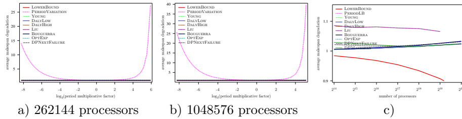
Figure 87: Evaluation of the different heuristics on a Exascale platform with Exponential failures ( MTBF = 1250 years), using Numerical Kernel law with \gamma = 10 , and constant overhead model
