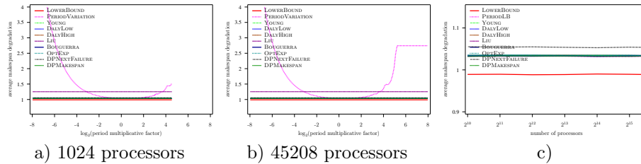
Figure 27: Evaluation of the different heuristics on a Petascale platform with Exponential failures ( MTBF = 500 years), using Amdahl law with \gamma = 10^{-6} , and variable overhead model ( C(p) = 600 \frac{45208}{p} )
