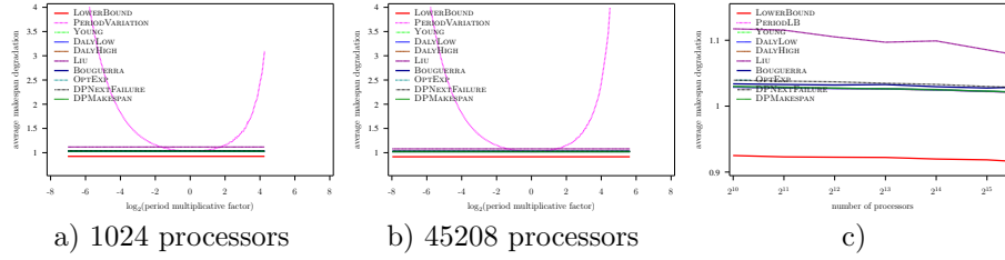
Figure 32: Evaluation of the different heuristics on a Petascale platform with Exponential failures ( MTBF = 125 years), using Numerical Kernel law with \gamma = 10 , and variable overhead model ( C(p) = 600 \frac{45208}{p} )
