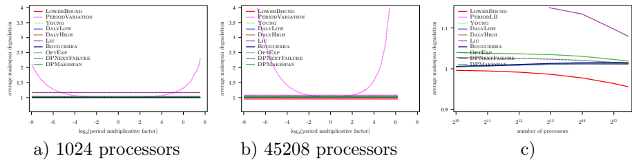
Figure 37: Evaluation of the different heuristics on a Petascale platform with Exponential failures ( MTBF = 500 years) using Amdahl law with \gamma = 10^{-4} , and constant overhead model
