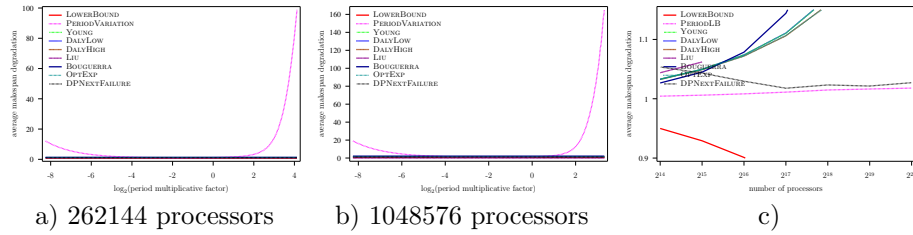
Figure 94: Evaluation of the different heuristics on a Exascale platform with Weibull failures ( MTBF = 1250 years), using Amdahl law with \gamma = 10^{-6} , and constant overhead model
