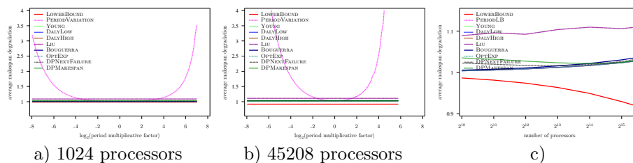
Figure 42: Evaluation of the different heuristics on a Petascale platform with Exponential failures ( MTBF = 125 years), using Numerical Kernel law with \gamma = 1 , and constant overhead model
