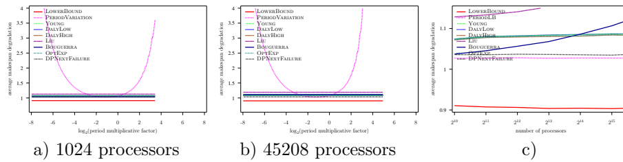
Figure 78: Evaluation of the different heuristics on a Petascale platform with Weibull failures ( MTBF = 500 years), using Numerical Kernel law with \gamma = 0.1 , and variable overhead model ( C(p) = 600 \frac{45208}{p} )
