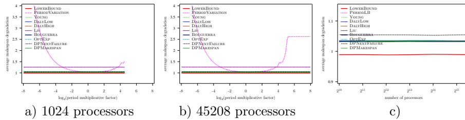
Figure 23: Evaluation of the different heuristics on a Petascale platform with Exponential failures ( MTBF = 500 years), using embarrassingly parallel job, and variable overhead model ( C(p) = 600 \frac{45208}{p} )
