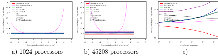
Figure 65: Evaluation of the different heuristics on a Petascale platform with Weibull failures ( MTBF = 500 years), using Numerical Kernel law with \gamma = 0.1 , and constant overhead model
