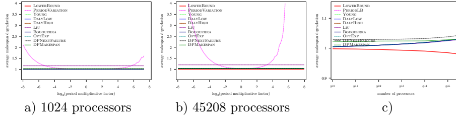
Figure 21: Evaluation of the different heuristics on a Petascale platform with Exponential failures ( MTBF = 500 years), using Numerical Kernel law with \gamma = 10 , and constant overhead model
