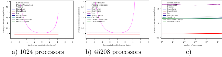
Figure 28: Evaluation of the different heuristics on a Petascale platform with Exponential failures ( MTBF = 125 years), using Numerical Kernel law with \gamma = 0.1 , and variable overhead model ( C(p) = 600 \frac{45208}{p} )
