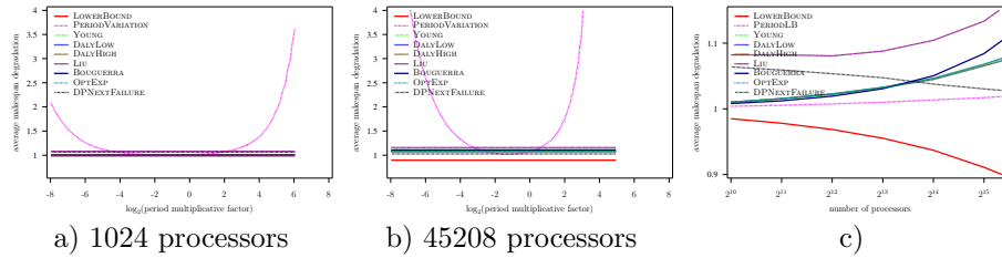
Figure 69: Evaluation of the different heuristics on a Petascale platform with Weibull failures ( MTBF = 500 years), using Numerical Kernel law with \gamma = 10 , and constant overhead model
