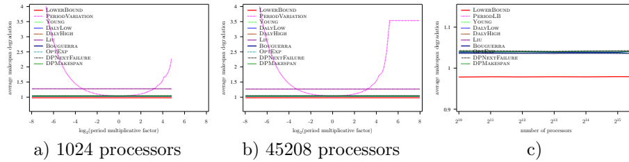
Figure 55: Evaluation of the different heuristics on a Petascale platform with Exponential failures ( MTBF = 500 years), using Numerical Kernel law with \gamma = 1 , and variable overhead model ( C(p) = 600 \frac{45208}{p} )
