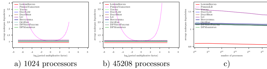
Figure 56: Evaluation of the different heuristics on a Petascale platform with Exponential failures ( MTBF = 125 years), using Numerical Kernel law with \gamma = 10 , and variable overhead model ( C(p) = 600 \frac{45208}{p} )
