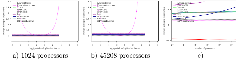
Figure 71: Evaluation of the different heuristics on a Petascale platform with Weibull failures ( MTBF = 500 years), using embarrassingly parallel job, and variable overhead model ( C(p) = 600 \frac{45208}{p} )
