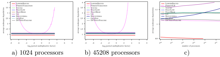
Figure 82: Evaluation of the different heuristics on a Petascale platform with Weibull failures ( MTBF = 500 years), using Numerical Kernel law with \gamma = 10 , and variable overhead model ( C(p) = 600 \frac{45208}{p} )
