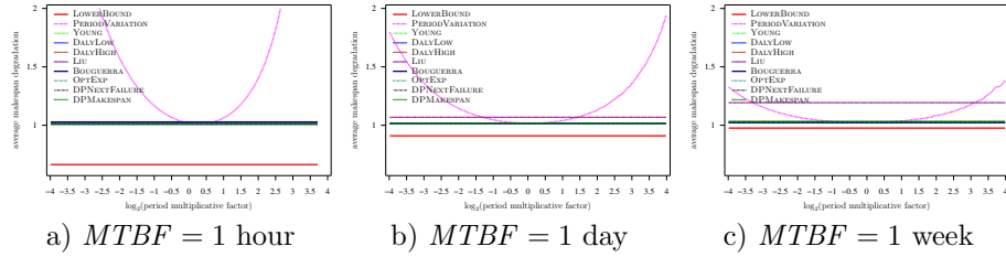
Figure 9: Evaluation of the different heuristics on one processor with Weibull failures ( k = 0.7 )
