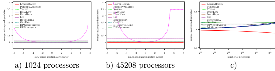
Figure 39: Evaluation of the different heuristics on a Petascale platform with Exponential failures ( MTBF = 500 years), using Amdahl law with \gamma = 10^{-6} , and constant overhead model
