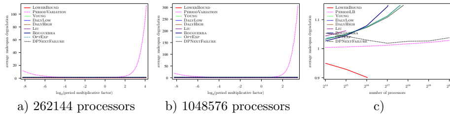
Figure 95: Evaluation of the different heuristics on a Exascale platform with Weibull failures ( MTBF = 1250 years), using Numerical Kernel law with \gamma = 0.1 , and constant overhead model
