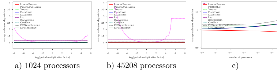
Figure 19: Evaluation of the different heuristics on a Petascale platform with Exponential failures ( MTBF = 500 years), using Numerical Kernel law with \gamma = 1 , and constant overhead model
