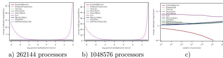
Figure 92: Evaluation of the different heuristics on a Exascale platform with Exponential failures ( MTBF = 1250 years), using Numerical Kernel law with \gamma = 10 , and constant overhead model
