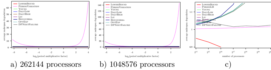
Figure 97: Evaluation of the different heuristics on a Exascale platform with Weibull failures ( MTBF = 1250 years), using Numerical Kernel law with \gamma = 10 , and constant overhead model
