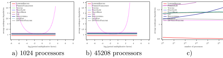
Figure 80: Evaluation of the different heuristics on a Petascale platform with Weibull failures ( MTBF = 500 years), using Numerical Kernel law with \gamma = 1 , and variable overhead model ( C(p) = 600 \frac{45208}{p} )
