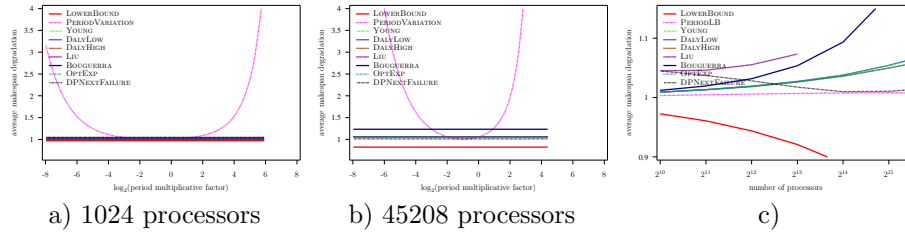
Figure 60: Evaluation of the different heuristics on a Petascale platform with Weibull failures ( MTBF = 125 years), using Amdahl law with \gamma = 10^{-4} , and constant overhead model
