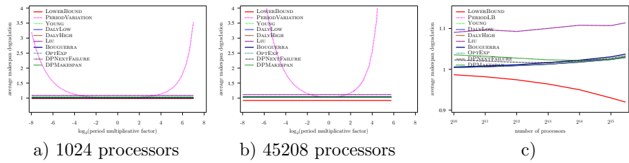
Figure 38: Evaluation of the different heuristics on a Petascale platform with Exponential failures ( MTBF = 125 years), using Amdahl law with \gamma = 10^{-6} , and constant overhead model
