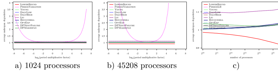
Figure 40: Evaluation of the different heuristics on a Petascale platform with Exponential failures ( MTBF = 125 years), using Numerical Kernel law with \gamma = 0.1 , and constant overhead model
