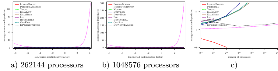
Figure 93: Evaluation of the different heuristics on a Exascale platform with Weibull failures ( MTBF = 1250 years), using embarrassingly parallel job, and constant overhead model
