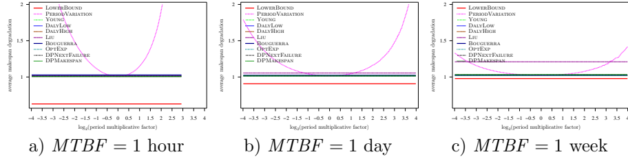
Figure 8: Evaluation of the different heuristics on one processor with Exponential failures
