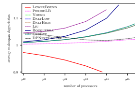
Figure 4: Evaluation of the different heuristics on a Petascale platform with Weibull failures.
