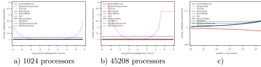
Figure 35: Evaluation of the different heuristics on a Petascale platform with Exponential failures ( MTBF = 500 years) using embarrassingly parallel job, and constant overhead model
