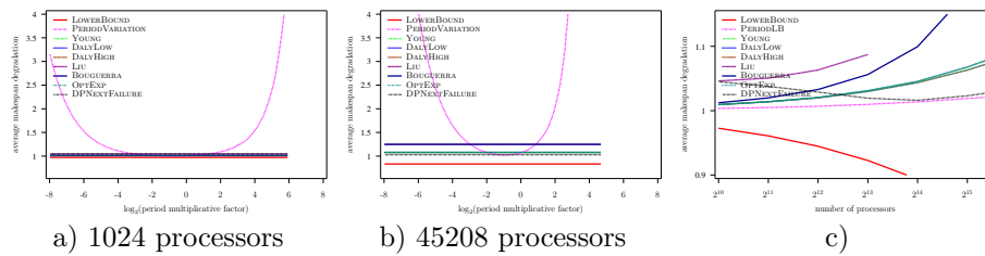
Figure 66: Evaluation of the different heuristics on a Petascale platform with Weibull failures ( MTBF = 125 years), using Numerical Kernel law with \gamma = 1 , and constant overhead model
