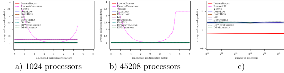
Figure 53: Evaluation of the different heuristics on a Petascale platform with Exponential failures ( MTBF = 500 years), using Numerical Kernel law with \gamma = 0.1 , and variable overhead model ( C(p) = 600 \frac{45208}{p} )
