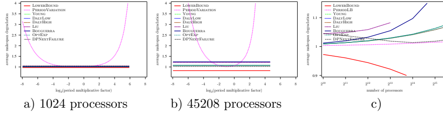
Figure 68: Evaluation of the different heuristics on a Petascale platform with Weibull failures ( MTBF = 125 years), using Numerical Kernel law with \gamma = 10 , and constant overhead model
