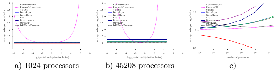
Figure 58: Evaluation of the different heuristics on a Petascale platform with Weibull failures ( MTBF = 125 years), using embarrassingly parallel job, and constant overhead model
