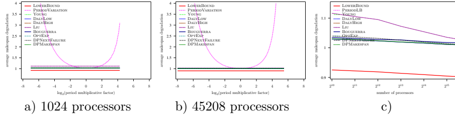
Figure 24: Evaluation of the different heuristics on a Petascale platform with Exponential failures ( MTBF = 125 years), using Amdahl law with \gamma = 10^{-4} , and variable overhead model ( C(p) = 600 \frac{45208}{p} )
