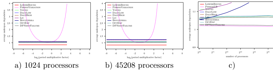
Figure 81: Evaluation of the different heuristics on a Petascale platform with Weibull failures ( MTBF = 125 years), using Numerical Kernel law with \gamma = 10 , and variable overhead model ( C(p) = 600 \frac{45208}{p} )
