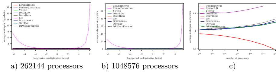
Figure 85: Evaluation of the different heuristics on a Exascale platform with Exponential failures ( MTBF = 1250 years), using Numerical Kernel law with \gamma = 0.1 , and constant overhead model
