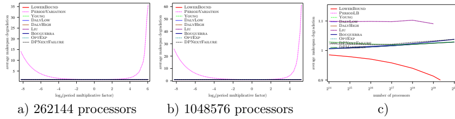
Figure 84: Evaluation of the different heuristics on a Exascale platform with Exponential failures ( MTBF = 1250 years), using Amdahl law with \gamma = 10^{-6} , and constant overhead model
