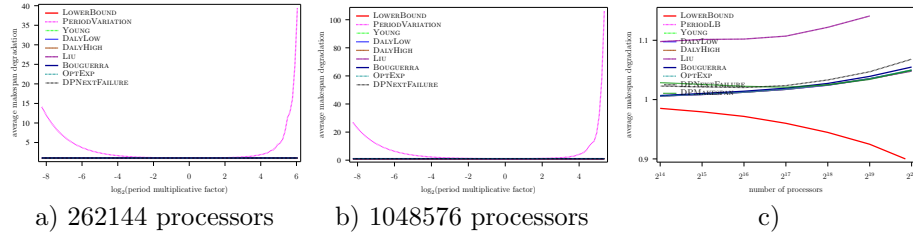
Figure 83: Evaluation of the different heuristics on a Exascale platform with Exponential failures ( MTBF = 1250 years), using embarrassingly parallel job, and constant overhead model
