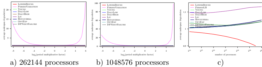
Figure 88: Evaluation of the different heuristics on a Exascale platform with Exponential failures ( MTBF = 1250 years), using embarrassingly parallel job, and constant overhead model
