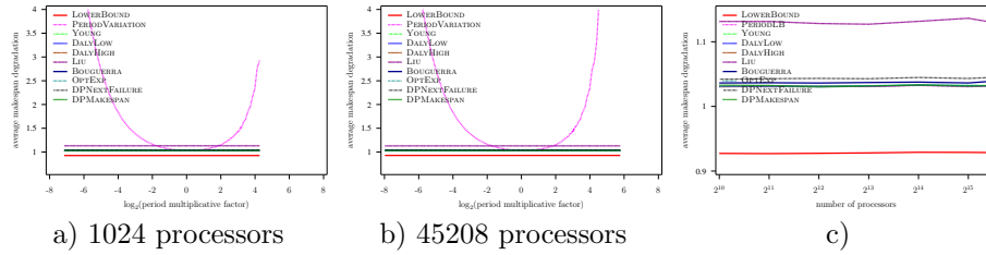
Figure 22: Evaluation of the different heuristics on a Petascale platform with Exponential failures ( MTBF = 125 years), using embarrassingly parallel job, and variable overhead model ( C(p) = 600 \frac{45208}{p} )
