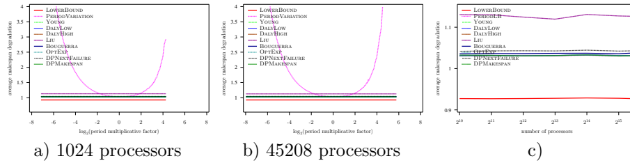
Figure 26: Evaluation of the different heuristics on a Petascale platform with Exponential failures ( MTBF = 125 years), using Amdahl law with \gamma = 10^{-6} , and variable overhead model ( C(p) = 600 \frac{45208}{p} )
