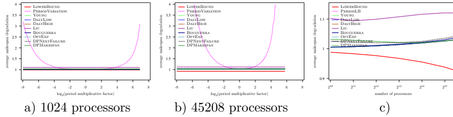
Figure 18: Evaluation of the different heuristics on a Petascale platform with Exponential failures ( MTBF = 125 years), using Numerical Kernel law with \gamma = 1 , and constant overhead model
