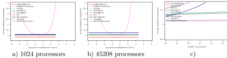
Figure 70: Evaluation of the different heuristics on a Petascale platform with Weibull failures ( MTBF = 125 years), using embarrassingly parallel job, and variable overhead model ( C(p) = 600 \frac{45208}{p} )
