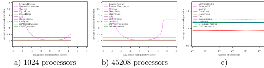
Figure 29: Evaluation of the different heuristics on a Petascale platform with Exponential failures ( MTBF = 500 years), using Numerical Kernel law with \gamma = 0.1 , and variable overhead model ( C(p) = 600 \frac{45208}{p} )
