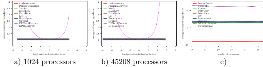
Figure 46: Evaluation of the different heuristics on a Petascale platform with Exponential failures ( MTBF = 125 years), using embarrassingly parallel job, and variable overhead model ( C(p) = 600 \frac{45208}{p} )
