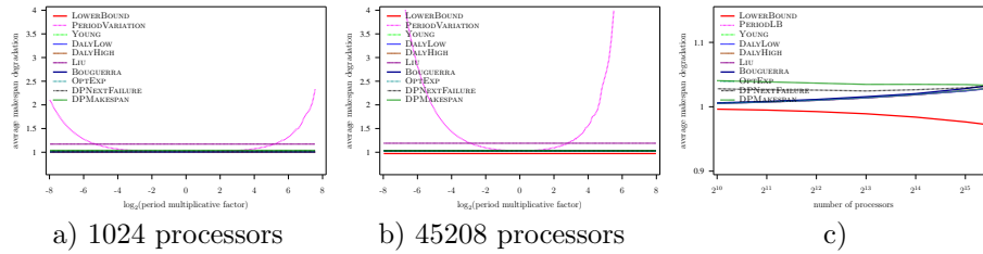
Figure 45: Evaluation of the different heuristics on a Petascale platform with Exponential failures ( MTBF = 500 years), using Numerical Kernel law with \gamma = 10 , and constant overhead model
