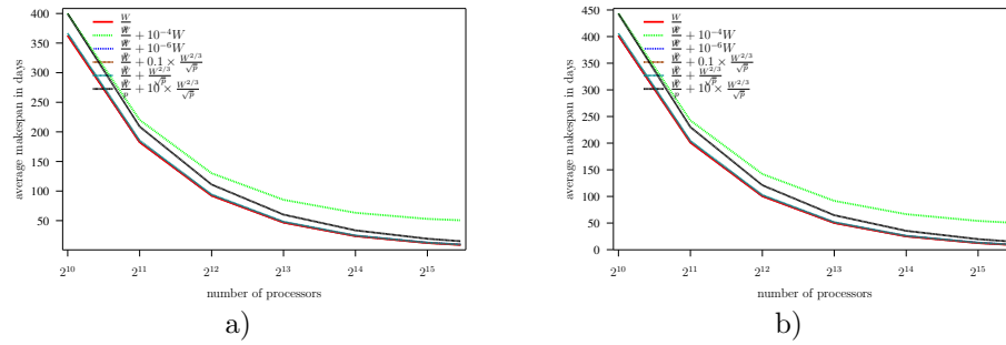
Figure 98: Evolution of the makespan for OPTEXP as a function of the platform size for the different application profiles and a constant (a) or platform-dependent (b) checkpoint cost (exponential law, MTBF = 125 years).
