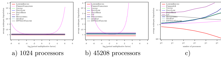
Figure 67: Evaluation of the different heuristics on a Petascale platform with Weibull failures ( MTBF = 500 years), using Numerical Kernel law with \gamma = 1 , and constant overhead model
