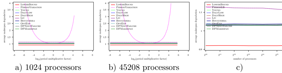
Figure 52: Evaluation of the different heuristics on a Petascale platform with Exponential failures ( MTBF = 125 years), using Numerical Kernel law with \gamma = 0.1 , and variable overhead model ( C(p) = 600 \frac{45208}{p} )
