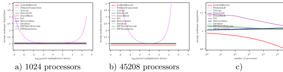
Figure 12: Evaluation of the different heuristics on a Petascale platform with Exponential failures ( MTBF = 125 years) using Amdahl law with \gamma = 10^{-4} , and constant overhead model
