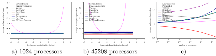
Figure 63: Evaluation of the different heuristics on a Petascale platform with Weibull failures ( MTBF = 500 years), using Amdahl law with \gamma = 10^{-6} , and constant overhead model
