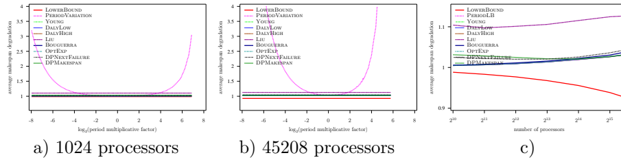
Figure 14: Evaluation of the different heuristics on a Petascale platform with Exponential failures ( MTBF = 125 years), using Amdahl law with \gamma = 10^{-6} , and constant overhead model
