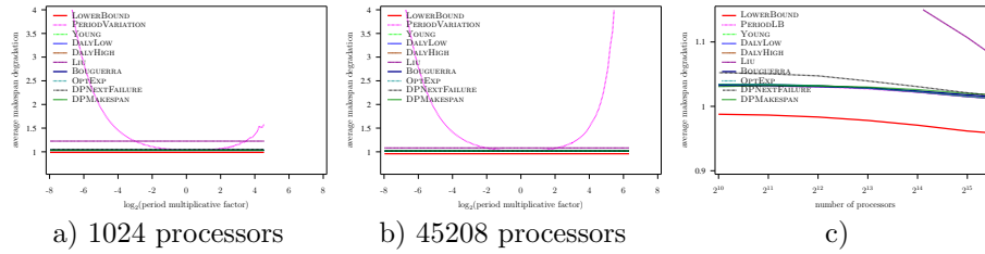
Figure 25: Evaluation of the different heuristics on a Petascale platform with Exponential failures ( MTBF = 500 years), using Amdahl law with \gamma = 10^{-4} , and variable overhead model ( C(p) = 600 \frac{45208}{p} )
