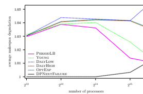
Figure 7: Evaluation of the different heuristics on a Petascale platform with failures based on the failure log of LANL cluster 19.
