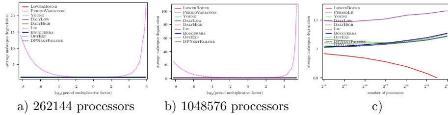
Figure 90: Evaluation of the different heuristics on a Exascale platform with Exponential failures ( MTBF = 1250 years), using Numerical Kernel law with \gamma = 0.1 , and constant overhead model
