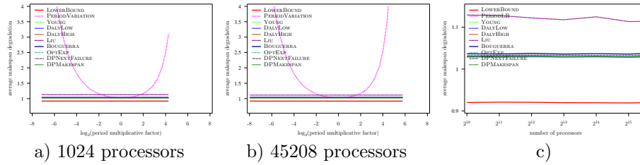
Figure 50: Evaluation of the different heuristics on a Petascale platform with Exponential failures ( MTBF = 125 years), using Amdahl law with \gamma = 10^{-6} , and variable overhead model ( C(p) = 600 \frac{45208}{p} )
