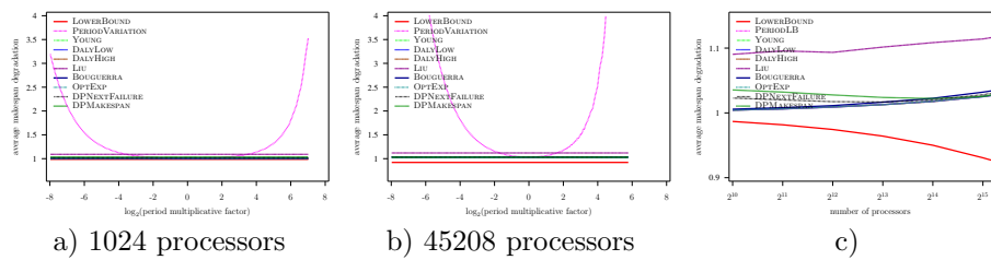
Figure 34: Evaluation of the different heuristics on a Petascale platform with Exponential failures ( MTBF = 125 years) using embarrassingly parallel job, and constant overhead model
