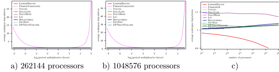
Figure 89: Evaluation of the different heuristics on a Exascale platform with Exponential failures ( MTBF = 1250 years), using Amdahl law with \gamma = 10^{-6} , and constant overhead model
