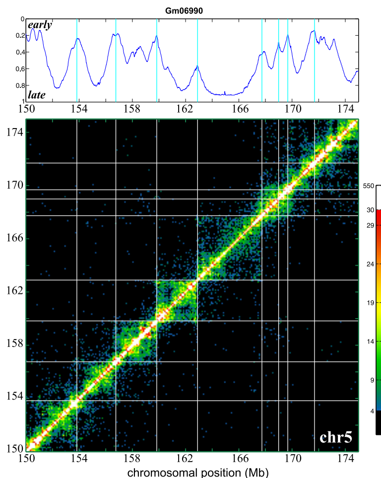
Figure 47: (suppl.) Replication domains correspond to structural self-interacting domains. Hi-C proximity heat-map for the intra-chromosomal interactions in Gm06990 cells on the chr5:150-175Mb locus. Each pixel represents the interaction in a 100 kb window. The colormap represents the number of reads for every pixel. A replication domain delimited by two local timing peaks corresponds to a self-interacting domain in Hi-C data, indicating that the timing peaks delineate the frontiers of megabase-sized structural domains.
