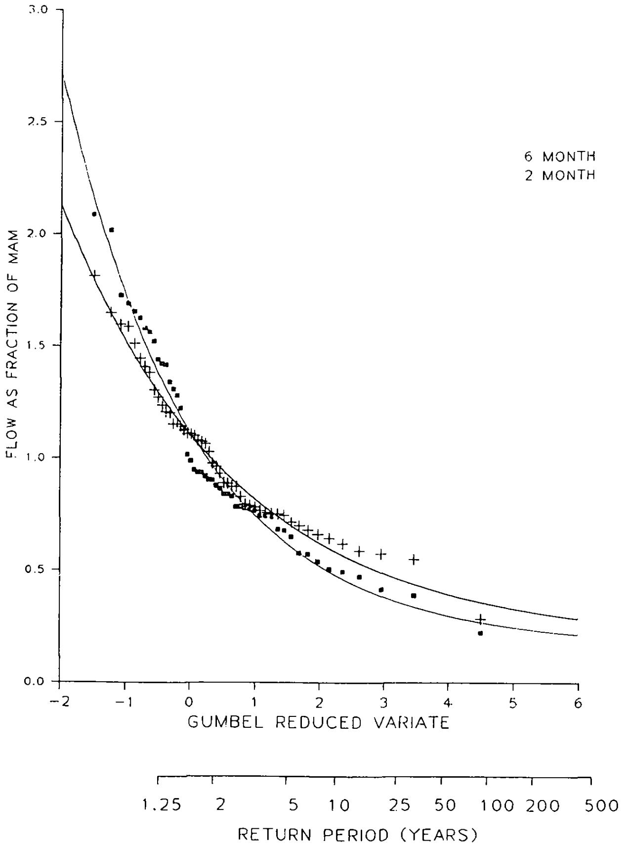
Figure 14 Annual minimum curve defined by a Weibull fit to the extended Annan record for 2 and 6 month durations
