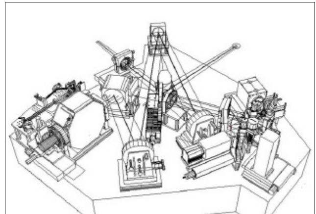
This is a drawing of the adaptive optics system of the Keck-2 telescope. As you can see, it is very complicated--but the activities you have just done still show the basic idea.
