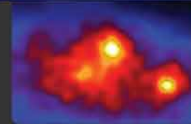
Brighter colors in the Cygnus region indicate greater numbers of gamma rays detected by the Fermi gamma ray space telescope.
