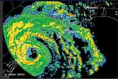
This Doppler-radar image seen on TV weather news uses microwaves for local weather forecasting. Shown here is Hurricane Claudette's eye wall making landfall.
