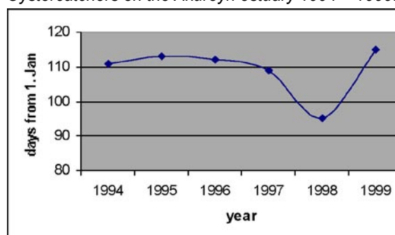
Figure EA-BI-8: Day of maximum number of Oystercatchers on the Akureyri estuary 1994 – 1999.
