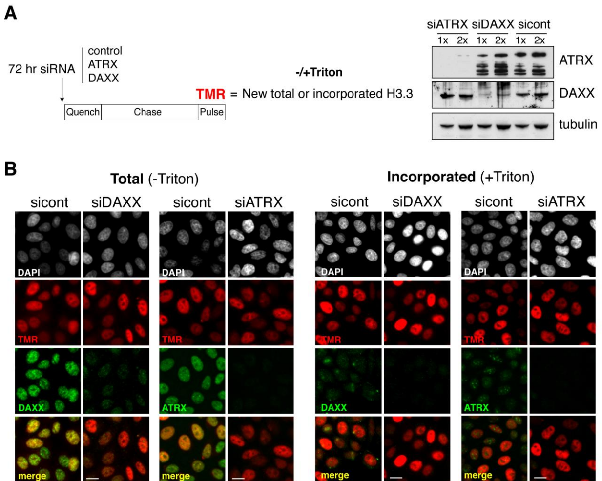
Figure S5 (related to main figure 4)
