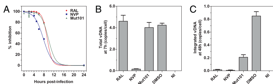
Figure 5 Time of addition experiment and qPCR analysis. (A) Time-of-addition (TOA) experiment in single-round infection assay of MT4 cells infected with VSV-G-pseudotyped HIV-1 \Delta env-Luc NL4-3. Each compound (Mut101, Nevirapine (NVP) or Raltegravir (RAL)) was added at the indicated times post-infection. Infection was measured by luciferase assays. Relative inhibition (%) was determined by comparison with the control. qPCR analysis of (B) the formation of proviral DNA at reverse transcription, and (C) the integration of the proviral DNA in the host cell genome after compound treatment as indicated. NI: not infected. Data represent the means of quadruplicates with standard deviations shown as error bars.
