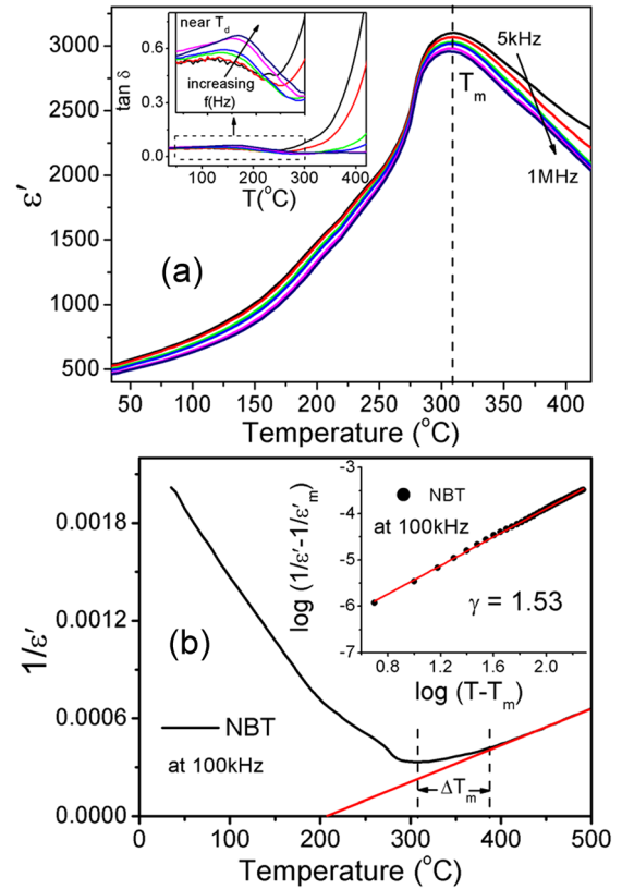
FIG. 6. (a) \epsilon' vs. T ( ^{\circ}\text{C} ) plot depicting diffused phase transition near T_m (i.e., \cong 310 ^{\circ}\text{C} for 100 kHz data) along with \tan\delta vs. T ( ^{\circ}\text{C} ) in the inset of Fig. 6(a). (b) Curie-Weiss ( 1/\epsilon' vs T ( ^{\circ}\text{C} )) and diffusivity plots (inset of Fig. 6(b)) indicating the relaxor behavior of NBT.
