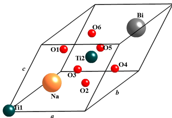
FIG. 1. The rhombohedral ( R3c ) unit cell of NBT. The lattice constant, angle, and the structural parameters are given in Table I.
