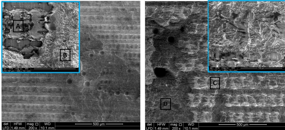
Figure 23 - SEM images of laser ablated ( ED=0.51 \text{ J/mm}^2 , H=100 \mu\text{m} ) aluminum joint subjected to aging method C ((i) left side; (ii) right side), with magnified details (in the blue boxes).
