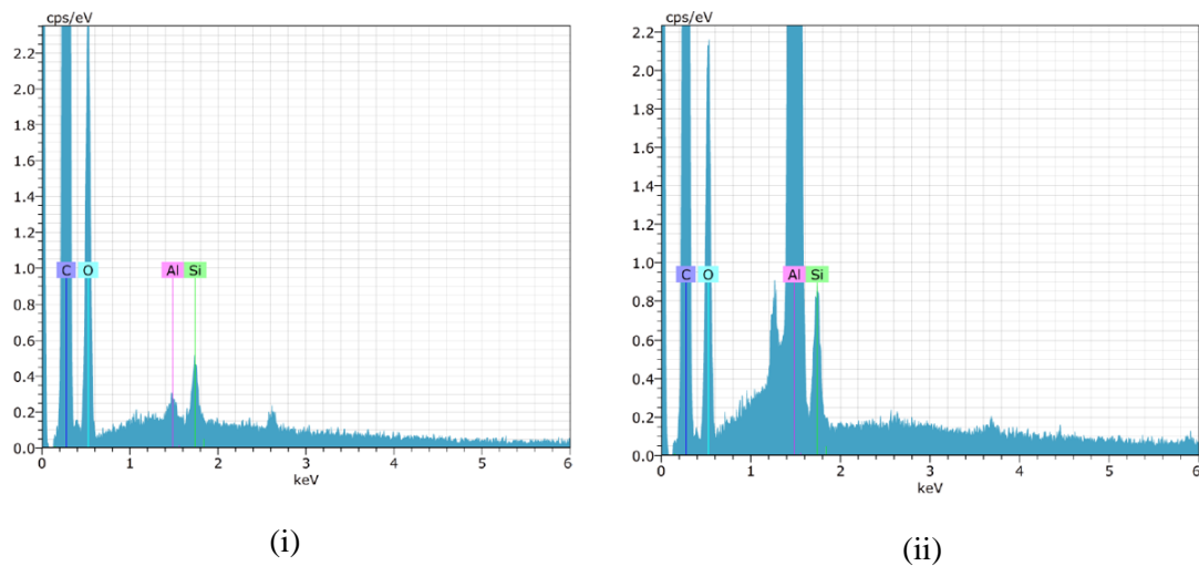
Figure 10 - Global EDX spectra measured on the observed surface showns in Figure 9(i) and (ii), respectively
