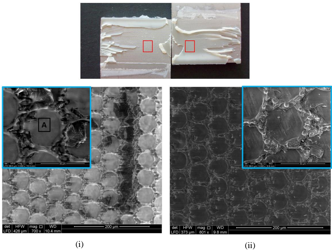
Figure 33 - SEM images of laser ablated ( ED=0.17 \text{ J/mm}^2 , H=50 \mu\text{m} ) stainless steel joint subjected to aging method C((i) left side; (ii) right side),
