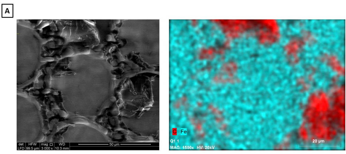
Figure 34 - Local EDX maps of the area A belonging to the surface shown in Figure 32
