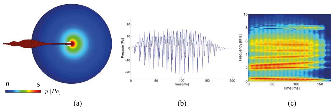
Fig. 1 – Finite element numerical simulation of diphthong /ei/. (a) Snapshot of the acoustic pressure during the articulation of vowel /i/, (b) acoustic pressure evolution at the mouth exit, (c) and spectrogram of (b).
