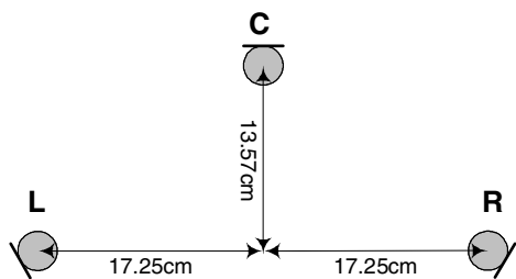
Figure 2.1: Configuration of microphone array 1: the angle between L and R is 100^\circ .
