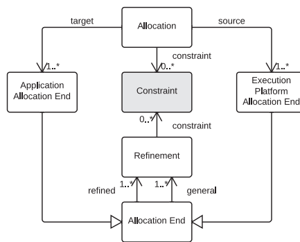
Figure A.7: UML MARTE - Allocation
