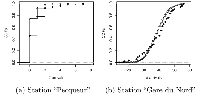
Figure 4: Comparisons between the theoretical (white dots) and empirical (black dots) CDFs for bike arrivals at two stations, in time window 6. The K-S test statistic is the maximum (vertical) distance between a pair of white and black dots in the graphs. The station on the left has a higher K-S test statistic ( K = 0.3815 ) than the one on the right ( K = 0.1633 ). There were 53 total arrivals at Pecqueur in this time window throughout the observation period, and 2186 at Gare du Nord (2187 if we account for a brief period of station fullness).
