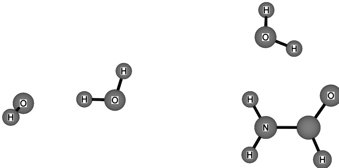
Scheme 1 : Equilibrium structures of the water dimer and the formamide-water complex.
