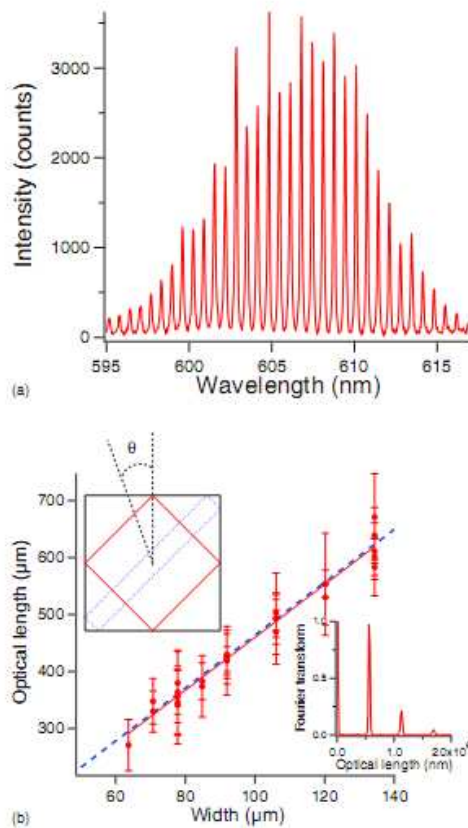
Figure 9 : optical spectrum obtained from a square-shaped PMMA:DCM microlaser (square width W=150 \mu\text{m} ), from ref.[119] (b) : a Fourier transform (inset) of the spectrum allows inferring directly the length of the periodic orbit, which as expected is found to vary linearly with the square dimension W . Reprinted figure with permission from [119]. Copyright 2011 by the American Physical Society.
