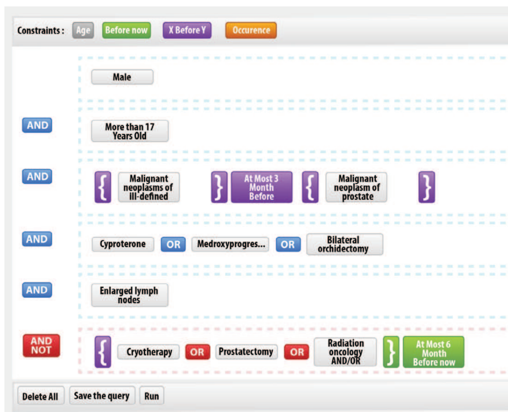
Figure 5: PFS query builder graphical user interface
