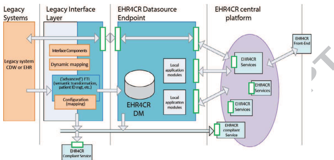
Figure 1: Simplified view of the EHR4CR platform
