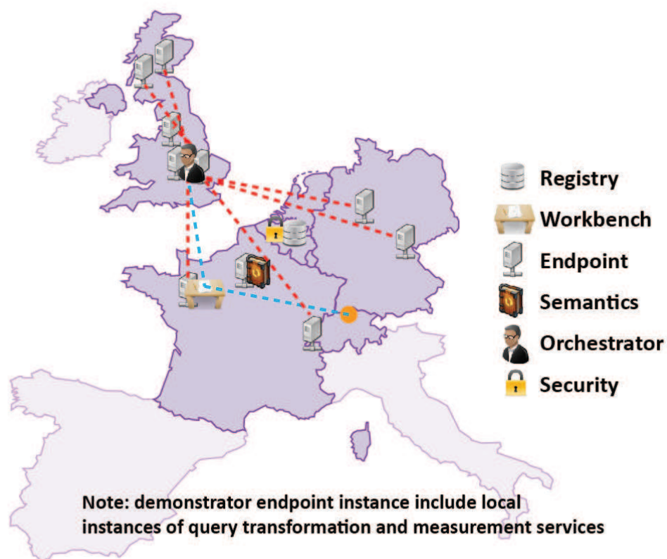
Figure 2: Overview of the main services of the Protocol Feasibility Scenario
