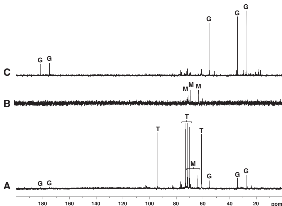
Figure 4 Natural abundance ^{13}\text{C} -NMR spectrum of major cytosolic solutes accumulated by R. etli wild-type and otsAch strains. Wild-type (A) and otsAch (B, C) cells were grown at 28°C in \text{B}^- minimal medium with 0.2 M NaCl. Cells were extracted as described in Materials and Methods. For the otsAch strain, cells were collected at the entrance of the first (B) and second (C) stationary phase of growth. The major solutes were trehalose (T), glutamate (G) and mannitol (M).
