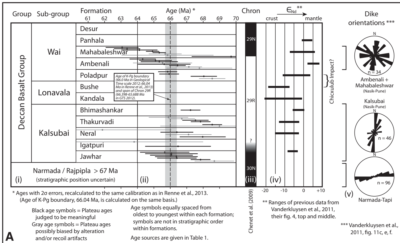
Figure 1. (A) (i) Deccan subgroups and formations (Chenet et al., 2008). Additional information includes (ii) radioisotopic ages (see Table 1 for sources) with 2\sigma uncertainties indicated by error bars, (iii) geomagnetic polarity assuming all reversed-polarity formations are within chron 29R, (iv) \epsilon_{Nd} ranges (Vanderkluyesen et al., 2011), and (v) orientations of associated dikes (Vanderkluyesen et al., 2011). Relatively minor-volume Narmada/Rajpipla basalts occurred during earlier phases of Deccan volcanism along the east-west Narmada Rift, and these clearly predate the Chicxulub impact. Gray area in column (ii) indicates approximate time range of chron 29R. (Continued on following page.)
