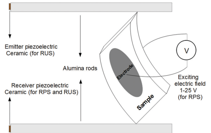
FIG. 2. (Color online) Schematic view of the experimental configuration used for resonant piezoelectric spectroscopy (RPS).
