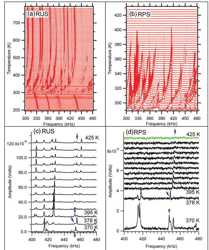
FIG. 4. (Color online) (a) RUS. (b) RPS spectra of \text{PbSc}_{0.5}\text{Ta}_{0.5}\text{O}_3 at high temperature. The left axis is the amplitude (in volts) but the spectra have been offset in proportion to the temperature at which they were collected. The axis is labeled accordingly. (c) Some RUS spectra collected between 370 and 425 K. (d) Some RPS spectra collected between 370 and 425 K. The blue arrows in (c) and (d) indicate the temperature evolution of the same sample resonance peak.
