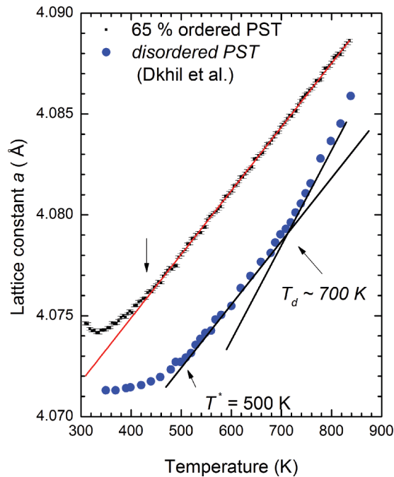
FIG. 3. (Color online) Temperature evolution of the pseudocubic lattice parameter of the reduced unit cell in the Fm\bar{3}m phase of \text{PbSc}_{0.5}\text{Ta}_{0.5}\text{O}_3 with Q_{\text{od}} = 0.65 . The red line is a linear fit to the data. The black arrow is placed at 425 K to indicate where the break from a linear trend occurs. Lattice parameter data for \text{PbSc}_{0.5}\text{Ta}_{0.5}\text{O}_3 with an unspecified degree of order, from Dkhil et al. , 9 are included for comparison (filled blue circles).
