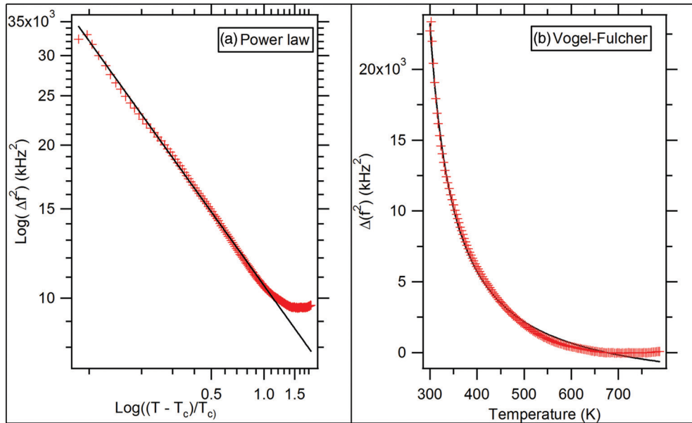
FIG. 8. (Color online) Temperature evolution of the squared frequency of the resonance frequency and the theoretical fits using (a) power law and (b) Vogel-Fulcher relation. For the power law, A_0(T - T_c)^x - B , the fit parameters are A_0 = 1.583210^5 kHz 2 , T_c = 275.85 K, \gamma = 0.48 , and B = 9607.6 kHz 2 . For Vogel-Fulcher relation, A_0 \exp(\frac{E_a}{T - T_{VF}}) - B , the fit parameters are A_0 = 17669 kHz 2 , T_{VF} = 220.38 K, E_a = 72.447 K, and B = 20719 kHz 2 . For (a) and (b), \Delta f^2 corresponds to the difference between the maximum value of the squared resonance frequency, f^2 = (115780) kHz 2 , obtained at 600–660 K and those obtained at temperatures between T_{trans} and 800 K. The coefficient B was used to compensate for the error in the baseline due to thermal expansion.
