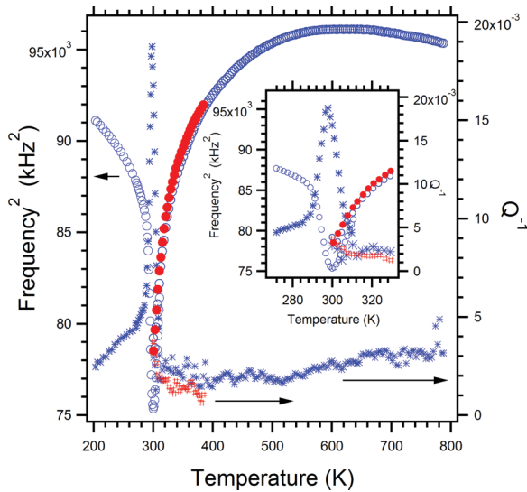
FIG. 5. (Color online) Temperature-dependence of the square of mechanical resonance frequencies and the inverse quality factor obtained for a single resonance peak from RUS and RPS spectra of \text{PbSc}_{0.5}\text{Ta}_{0.5}\text{O}_3 . RUS data for f^2 and Q^{-1} are shown with blue open circles and stars, respectively; RPS data are represented by red filled circles and number symbols.
