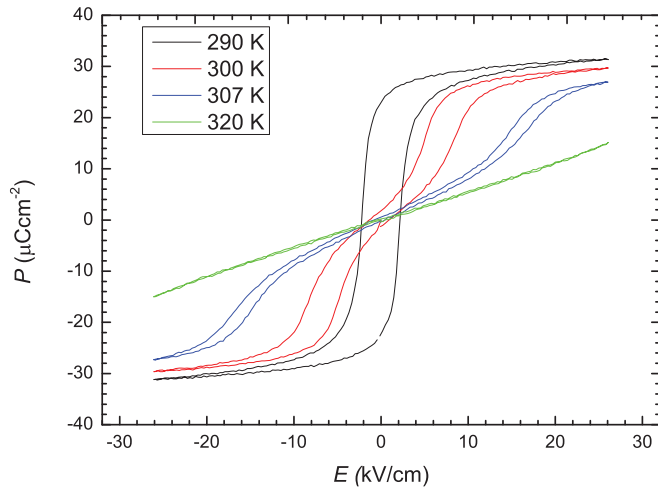
FIG. 7. (Color online) P(E) loops at 1 Hz obtained using a 420- \mu\text{m} -thick \text{PbSc}_{0.5}\text{Ta}_{0.5}\text{O}_3 sample at 290 (black line), 300 (red line), 307 (blue line), and 320 K (green line).
