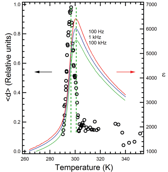
FIG. 6. (Color online) Variation of the space averaged piezoelectric coefficient \langle d \rangle (open circles) and dielectric constant, \epsilon , measured at 100 Hz, 1 kHz, and 100 kHz (red, blue, and green curves, respectively) with temperature across the cubic-rhombohedral phase transition. Maxima in \langle d \rangle and \epsilon occur at 296 and 300 K, respectively.
