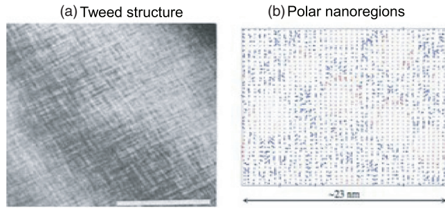
FIG. 1. (Color online) Comparison of tweed structures and polar nanoregions (PNRs). (a) An electron micrograph of tweed structures observed in \text{YBa}_2(\text{Cu}_{1-x}\text{Co}_x)_3\text{O}_{7-\delta} . Scale bar corresponds to 0.1 \mu\text{m} [reprinted by permission of the publisher 20 from Ref. 14]. (b) A simulation of PNR's. The horizontal dimension of the image corresponds to 23 \text{ nm} . [Reprinted with permission from Ref. 13. Copyright (2013) by the American Physical Society.]
