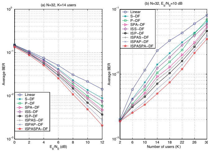
Fig. 4. BER performance versus (a) E_b/N_0 and (b) number of users (K).
