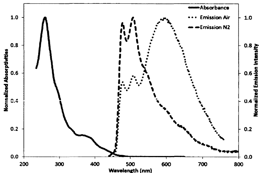
Figure A- 74 Absorption spectra (solid line), deaerated (dashed line) and aerated (dotted line) 298 K emission spectra respectively of [Ir(ppy) 2 (pythdo)] (86) in ACN.
