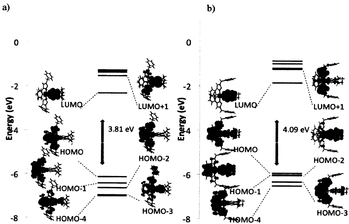
Figure A- 66 Kohn-Shan energy diagram for a) complex 80b and b) complex 80c.
