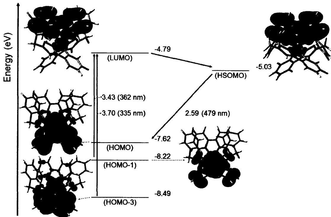
Figure A- 38. Jablonski diagram for complex 78a.
