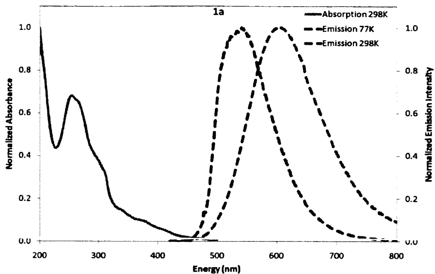
Figure A-28. Absorption and emission spectra for 1 [Ir(ppy) 2 bpy]PF 6 :
