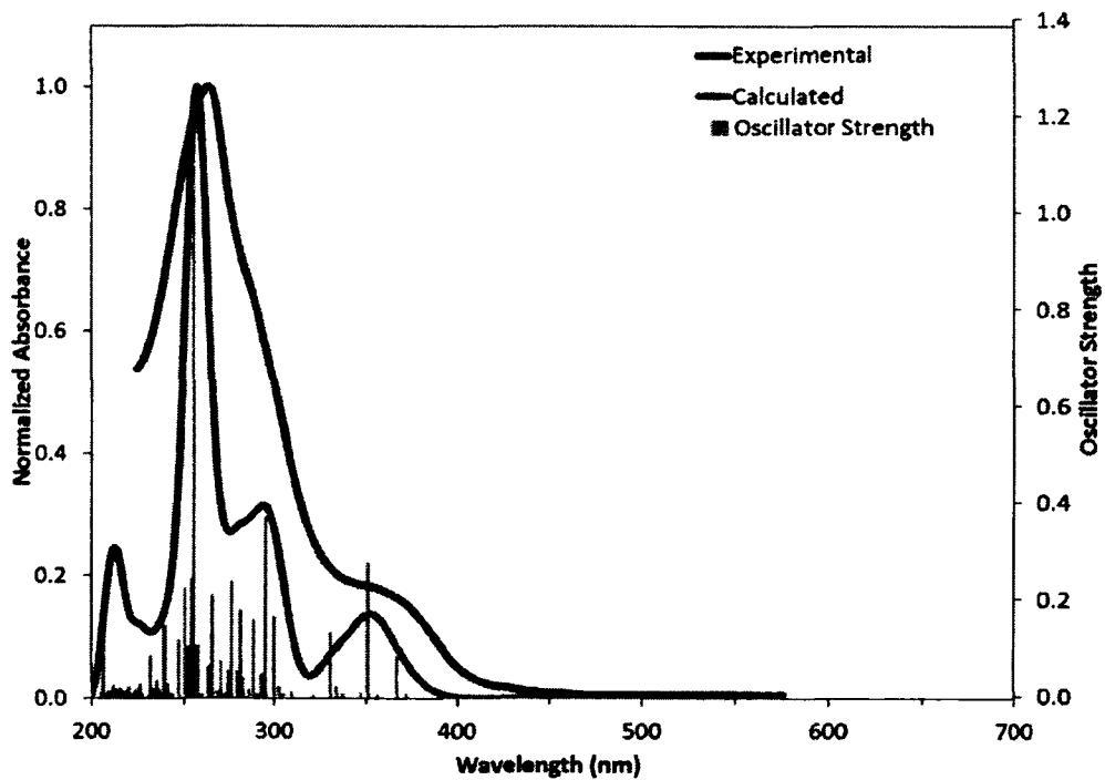
Figure A- 62 Calculated and experimental absorption spectra of 79b
