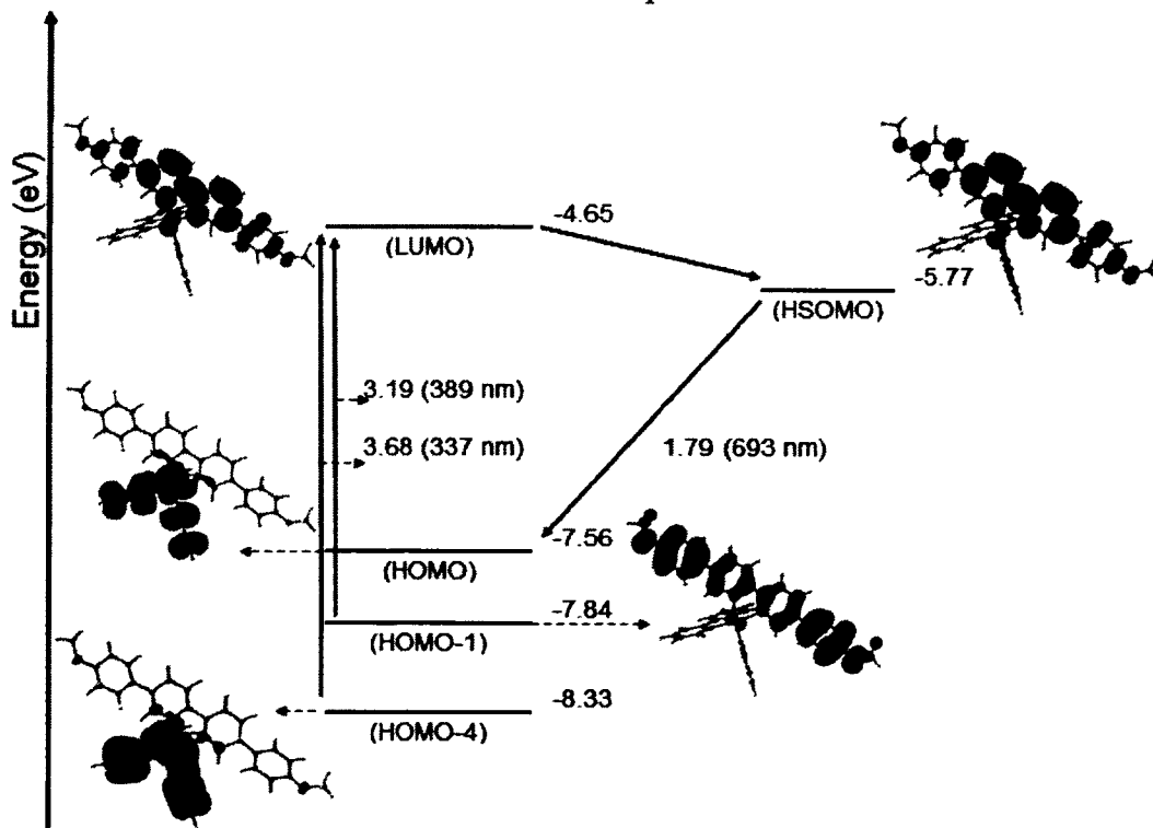
Figure A-15. State diagram and calculated molecular orbitals of major electronic transition for complex 10b.
