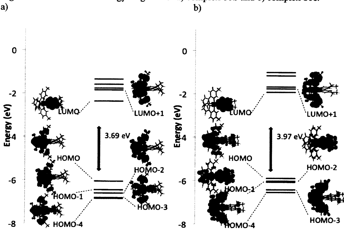
Figure A- 67 Kohn-Shan energy diagram for a) complex 79b and b) complex 79c
