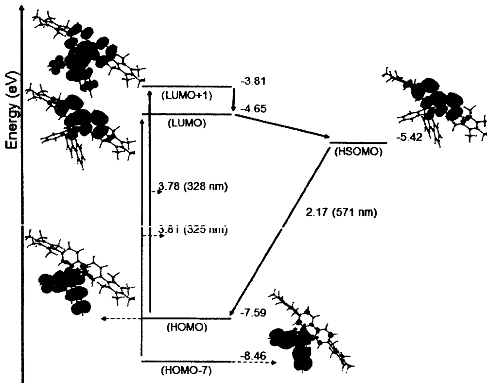
Figure A-20. State diagram and calculated molecular orbitals of major electronic transition for complex 10g .
