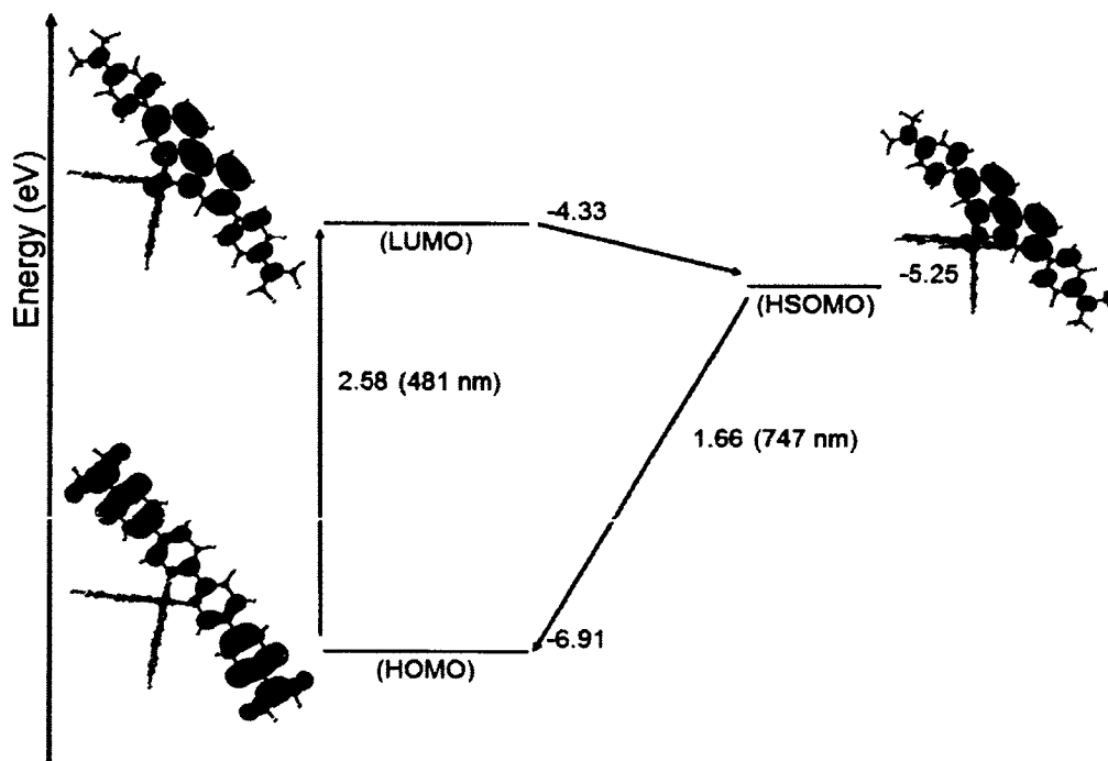
Figure A-16. State diagram and calculated molecular orbitals of major electronic transition for complex 10c.
