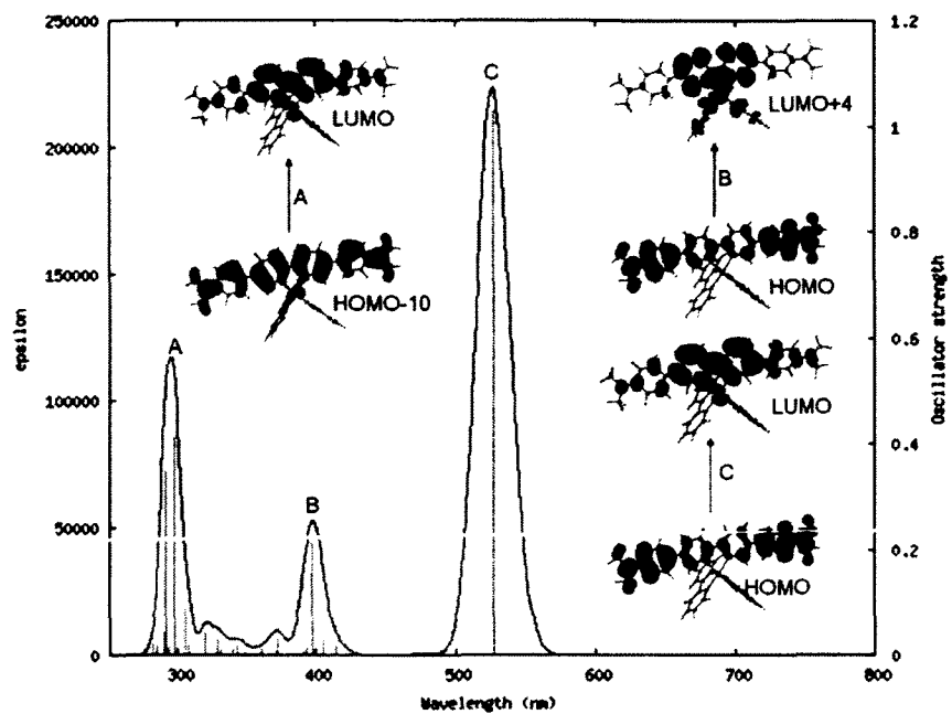
Figure A-24. Calculated absorption spectra of complex 10c .
