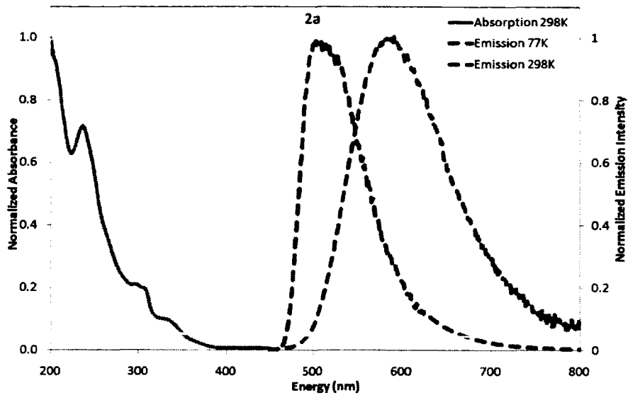
Figure A- 30. Absorption and emission spectra for 78a [\text{Ir}(\text{phtl})_2\text{bpy}]\text{PF}_6 .
