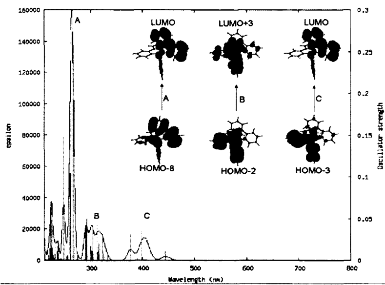
Figure S 29. Calculated absorption spectra of complex 1.
