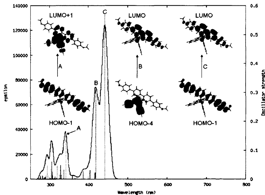
Figure A- 23. Calculated absorption spectra of complex 10b.
