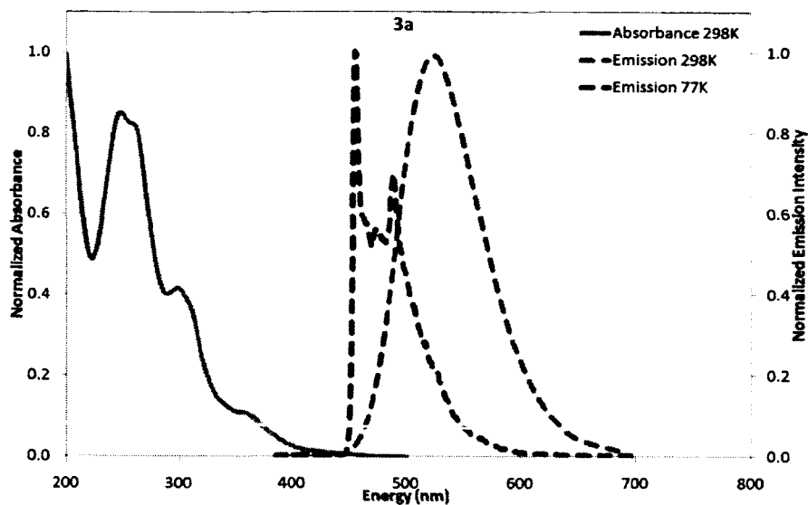
Figure A- 32. Absorption and emission spectra for 79a [\text{Ir}(\text{dFMeppy})_2\text{bpy}]\text{PF}_6
