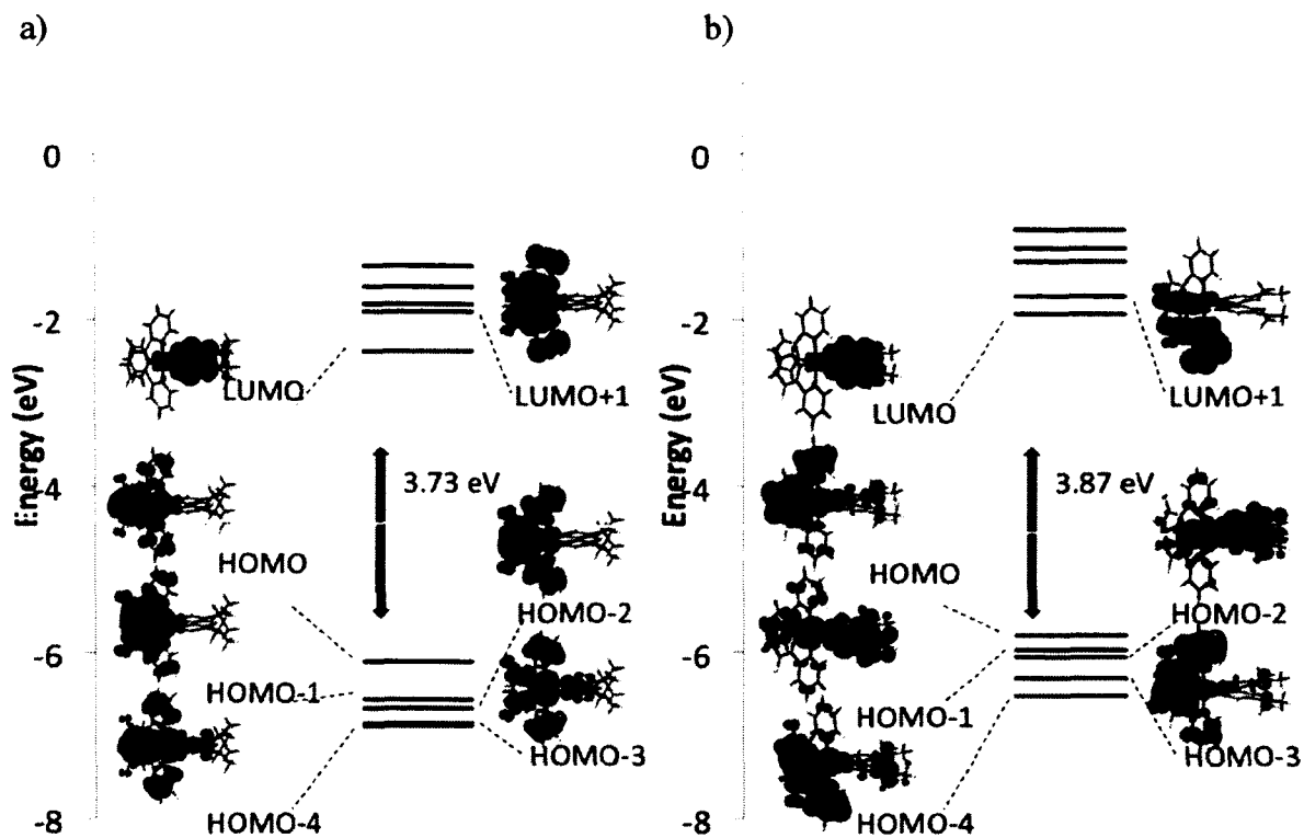
Figure A- 68. Kohn-Shan energy diagram for a) complex 81b and b) complex 81c
