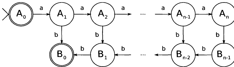
FIGURE 2.4 – DFA du langage a^n b^n
