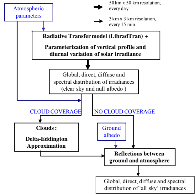
Figure 1. Heliosat-4 scheme
