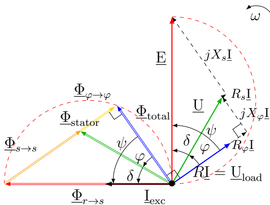
Figure A.7: Phasor representation of voltages and currents in the one-loop circuit. Single-line arrows represent voltages and currents, while double-line arrows stand for the flux density associated with the latter.
