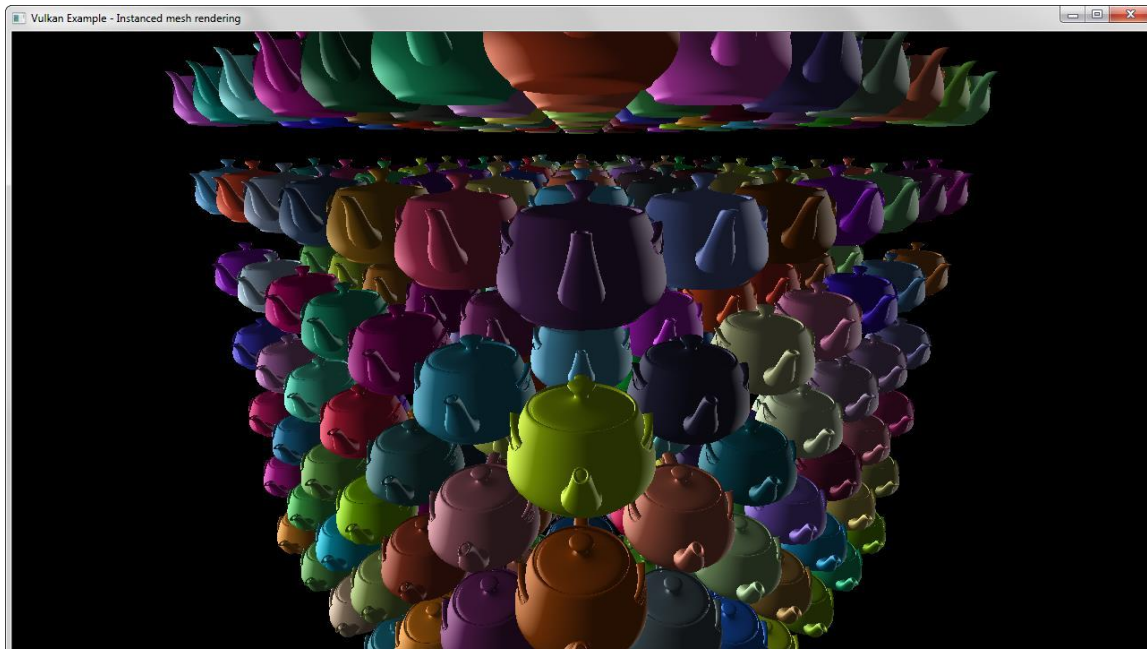
Figure 4.6 Mesh Instancing
