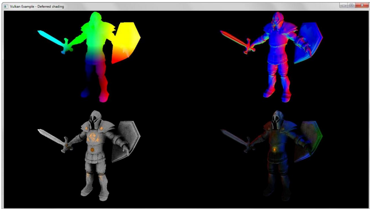
Figure 4.5 Deferred shading
