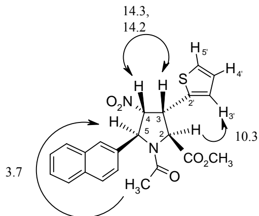
Figure 4. N.O.e. data of compound 16a
