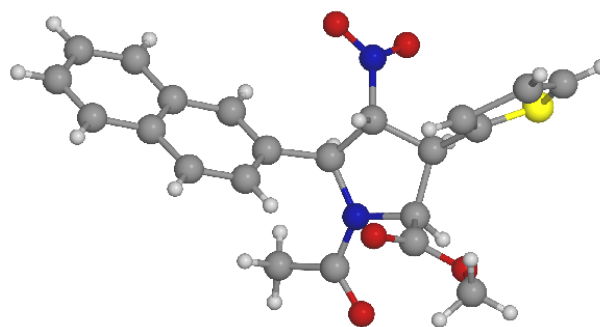
Figure 8: X-ray crystal structure of 16b
