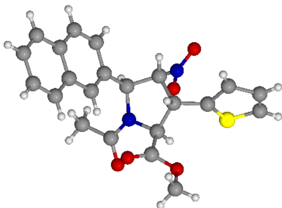
Figure 5: X-ray crystal structure of 16a
