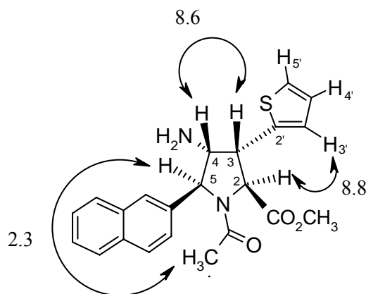
Figure 13. N.O.e. of compound 18a
