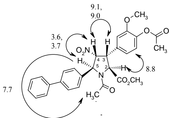
Figure 12. N.O.e. data of compound 17b
