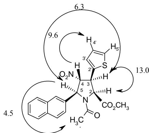
Figure 7. N.O.e. data of compound 16b
