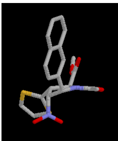
Figure 6. Stick model of 16a
