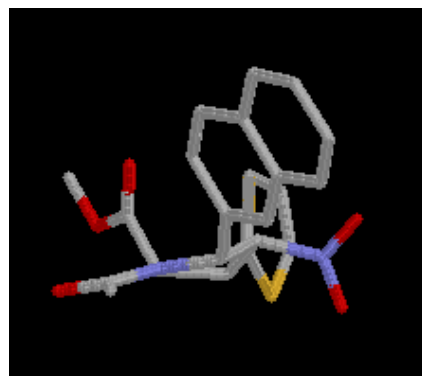
Figure 11. Model of 16b
