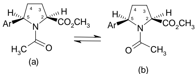
Figure 9. Two possible orientations of the N -acetyl
