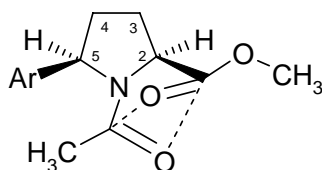
Figure 10. Possible dipole-dipole interaction
