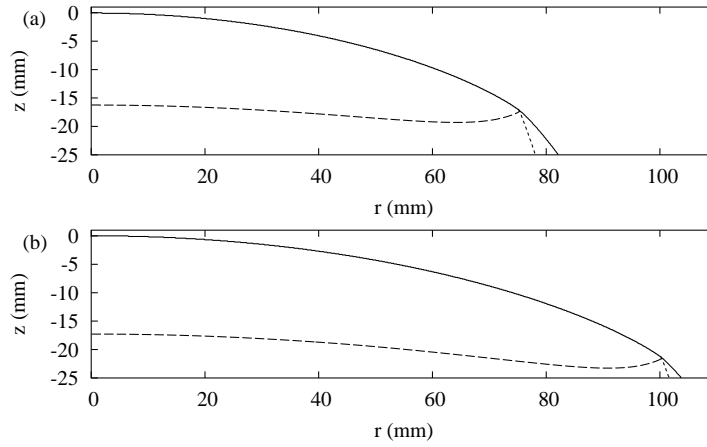
Figure 7. Shock locus (solid lines), sonic locus (dashed lines) and explosive/inert interface position (dotted lines) for \rho_I = 0.8 \text{ g/cm}^3 and (a) d = 150 \text{ mm} and (b) d = 200 \text{ mm} .
