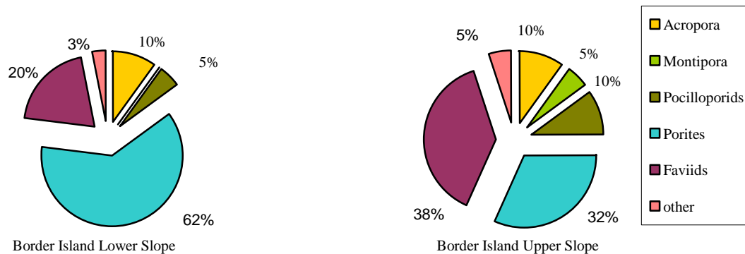
Figure 31. Coral community composition at Border Island at the time of surveys
