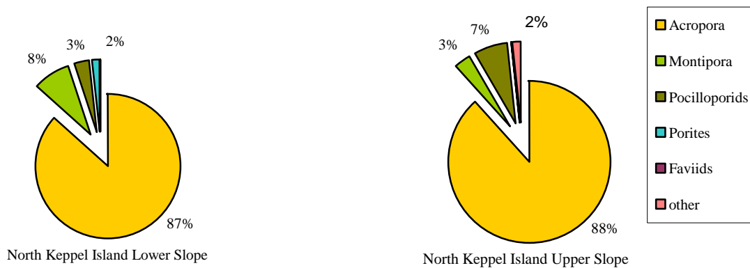
Figure 19. Coral community composition at North Keppel Island at the time of surveys
