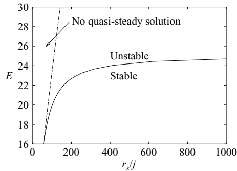
FIGURE 3. The neutral stability boundary from the linear stability analysis in Watt & Sharpe (2003). Also shown is the critical radius of curvature for the quasi-steady solutions (dashed line).
