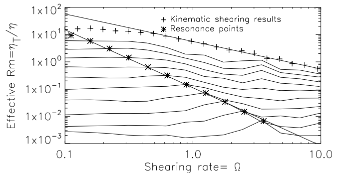
FIG. 6: The same as in Fig. 4 but with \tau_c \rightarrow 0 .
