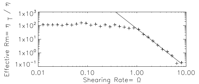
FIG. 3: R_m vs \Omega , clearly showing the transition at \Omega^{-1} = \tau_c = 1 ( B_0 = 0 )
