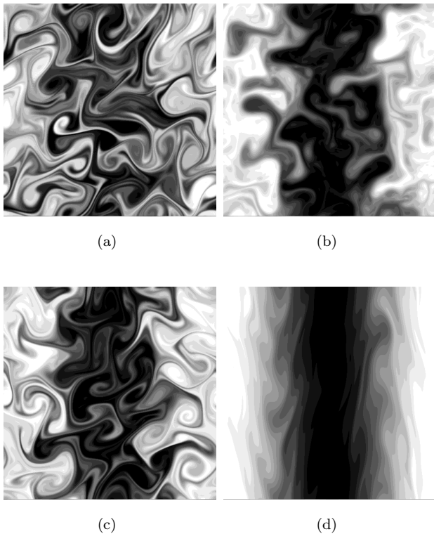
FIG. 1: Diffusion/mixing of A_0 for (a) M^2 \rightarrow \infty (B_0 = 0) and \Omega = 0 , (b) M^2 = 10 and \Omega = 0 , (c) M^2 \rightarrow \infty and \Omega = 1.0 , and (d) M^2 \rightarrow \infty and \Omega = 10 . All are taken at t = 5 with \tau_c = 1 .
