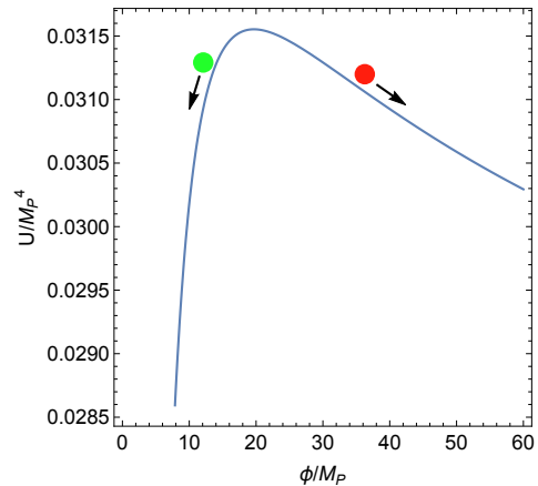
Figure 3: The non-minimally coupled potential for \delta = 0.1 , N_F = 10 , \xi = 1/6 , \mu_0 = 10^{-3} M_{\text{P}} .
