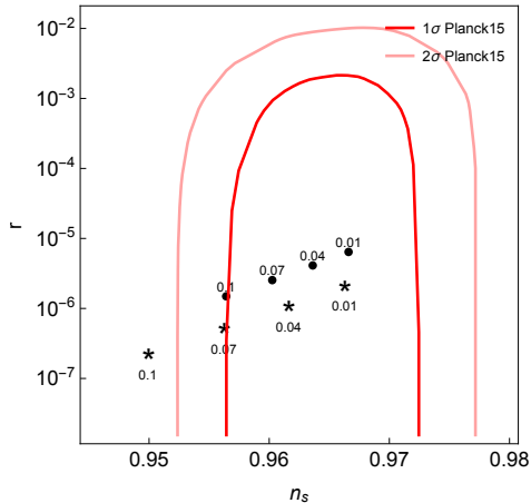
Figure 4: We compare the theoretical predictions in the r - n_s plane, in the non-minimally coupled case, for different values of \delta with Planck '15 results [51]. Full dots refer to the conformal coupling choice for \xi = 1/6 and the * marked points to \xi = 10^3 . We used the complete expression for the quantum corrected potential in (1) and further assumed \mu_0 = 10^{-3}M_P and the number of e -folds is 60.
