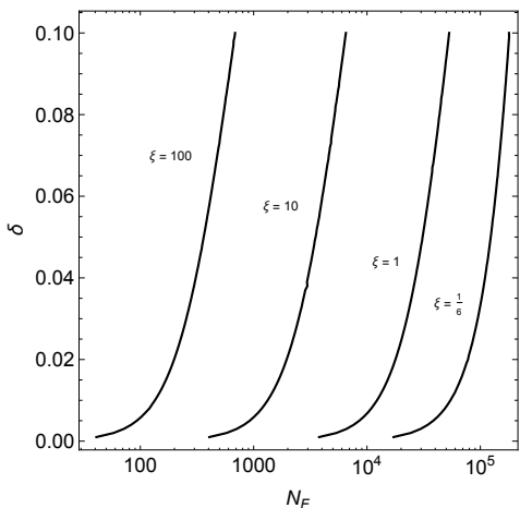
Figure 5: This figure shows the \delta dependence on N_F for different values of the non-minimal coupling \xi obtained by constraining the model to provide the observed amplitude of density perturbations. The plot assumes the transition scale \mu_0 = 10^{-3}M_P .
