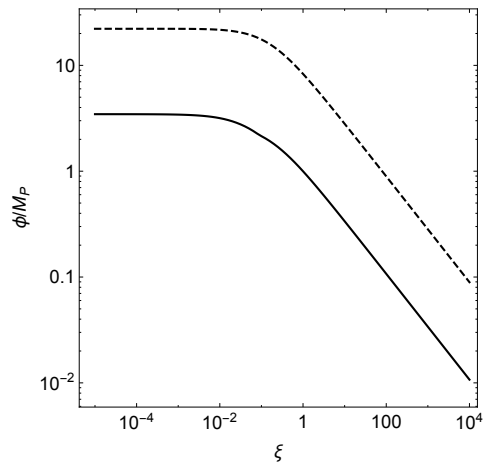
Figure 6: The figure shows the initial (dashed-line) and final (solid-line) values of the inflaton field in the Jordan frame as function of the non-minimal coupling \xi for \delta = 0.01 and \mu_0 = 10^{-3}M_P .
