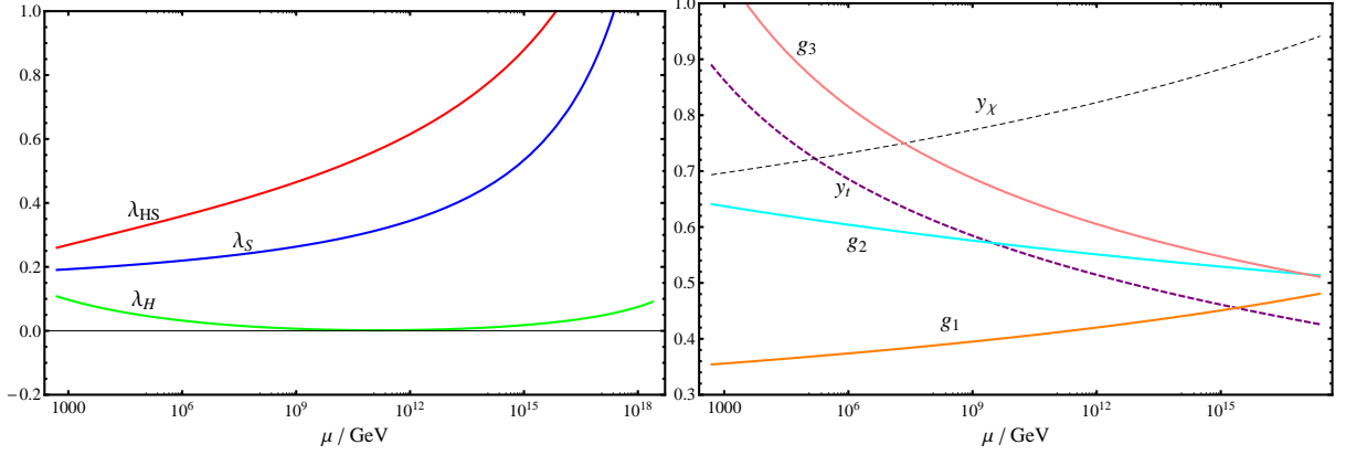
FIG. 1: RG evolution of the couplings, where Q_D = 1 , m_S = 500 GeV, \lambda_{HS}(m_S) = 0.26 , y_\chi(m_S) = 0.69 and \lambda_S(m_S) = 0.19 . The Higgs self coupling is stabilized due to the portal coupling \lambda_{HS} , which is here at its lower bound to ensure stability.
