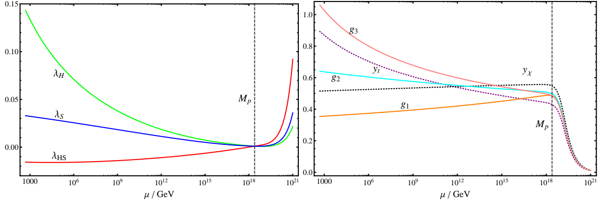
FIG. 4: RG evolution of the couplings, where we fixed Q_D = 1 and m_S = 500 GeV and used the Planck boundary conditions \lambda_H(M_P) \approx 0 , \lambda_{HS}(M_P) \approx 0 , \lambda_S(M_P) \approx 0 and y_\chi(M_P) = 0.54 , such that \beta_{\lambda_H}|_{M_P} \approx 0 and \beta_{\lambda_S}|_{M_P} \approx 0 . The numerical values for the gravity coefficient were taken universally to be \xi_0 = 0.024 , a_\lambda = 1 , a_y = -1 , and a_g = -1 . Large variations on these parameters have been investigated and no relevant differences were encountered.
