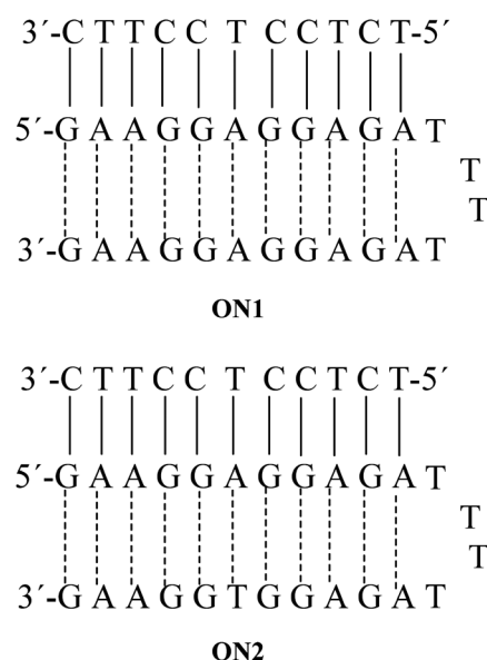
Fig. 3 Anti-parallel triplexes ON1 and ON2 .
