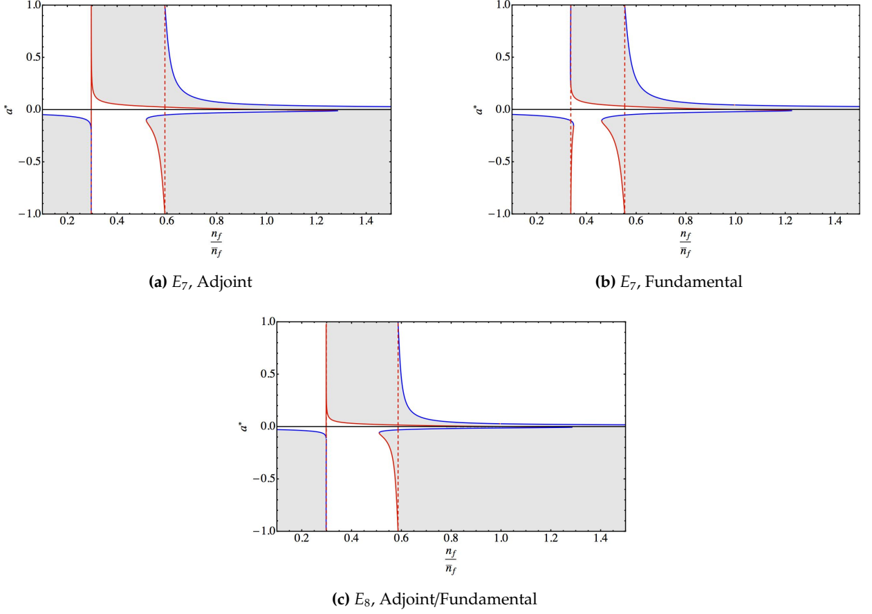
FIG. 5: Zerology to four loops for the given gauge groups and representations.
