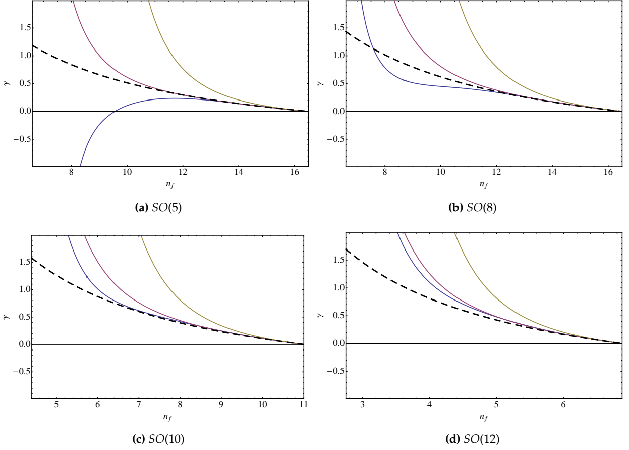
FIG. 8: Anomalous dimension at the perturbative fixed point as a function of number of flavors n_f for some SO(N) gauge group, illustrating the trend as N increases. The curve corresponding to i) two-loops is yellow, ii) three-loops is red, iii) four-loops is blue iv) all-orders is dashed.
