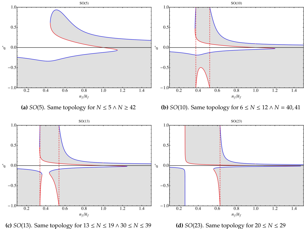
FIG. 3: The four distinct zerologies of SO(N) gauge theories, as found from the four loops beta functions. The particular groups shown are SO(5) , SO(10) , SO(13) and SO(23) . Red curves correspond to IR fixed point solutions for the given number of flavors, while blue curves correspond to UV fixed point solutions.
