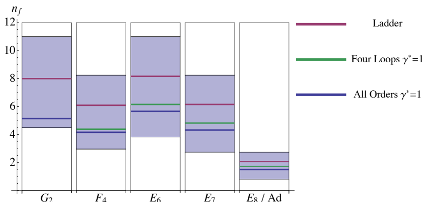
FIG. 1: For the exceptional groups we cannot change the number of colors and therefore the lines refer only to the number of flavors per given group. Therefore, we can only construct conformal lines in the flavor space. Nevertheless, we keep referring to them as conformal windows . We plot these lines as bars for the exceptional gauge theories with fermion matter transforming under the fundamental representation. The upper bound on the window is the asymptotic freedom limit, while the lower border is where the four loop fixed point is lost. The legend indicates the estimates from the methods described on the critical number of flavors where large distance conformality is lost. For E_8 the fundamental and adjoint are identical representations. The results for the theories with fermions in the adjoint representation are almost identical to the one of E_8 , as can be inspected from Table III.
