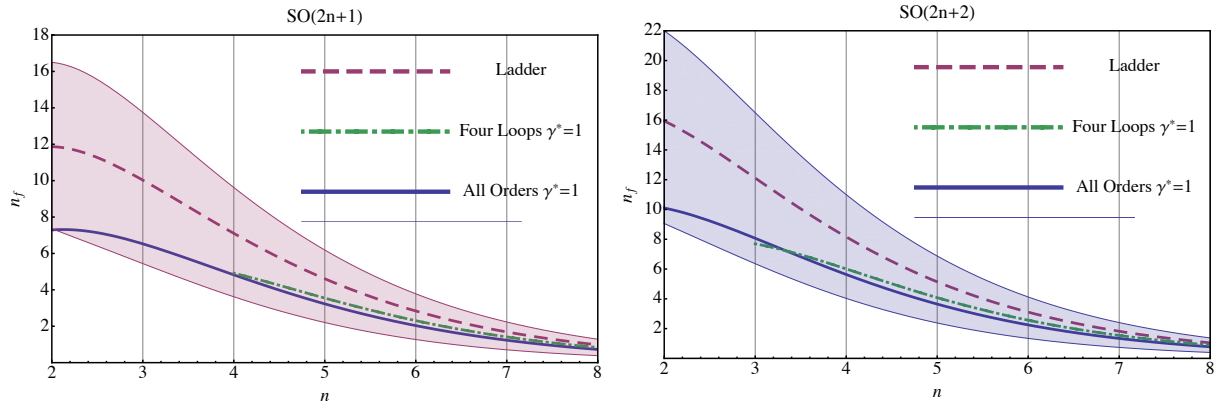
FIG. 2: Conformal window of SO(N) gauge theories with fermion matter transforming under the spinorial representation of the gauge group. The upper bound is the asymptotic freedom limit, while the lower border of the window is where the four loop fixed point is lost. The various estimates of the critical number of flavors where long distance conformality is lost, are shown as given by the legend. All estimates on the critical number of flavors has been determined by, or corresponds to, the value of the anomalous dimension being one, \gamma^* = 1 . Note that the four loops \gamma^* = 1 estimate is not applicable for SO(N < 8) . The all orders and four loop results are in surprisingly good agreement.
