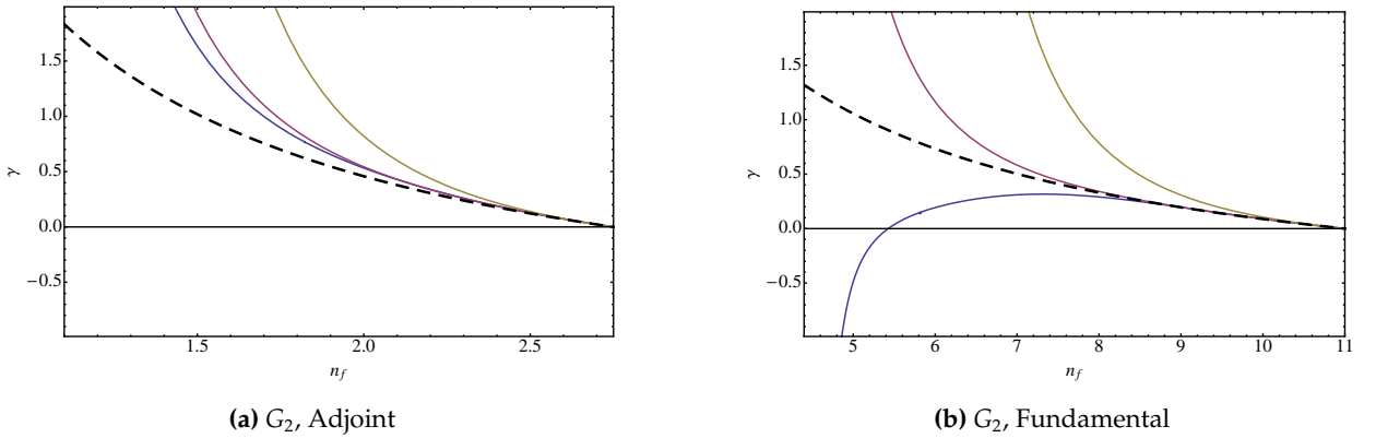
FIG. 6: Anomalous dimension at the perturbative fixed point as a function of number of flavors n_f . The curve corresponding to i) two loops is yellow, ii) three loops is red, iii) four loops is blue iv) all-orders is dashed.
