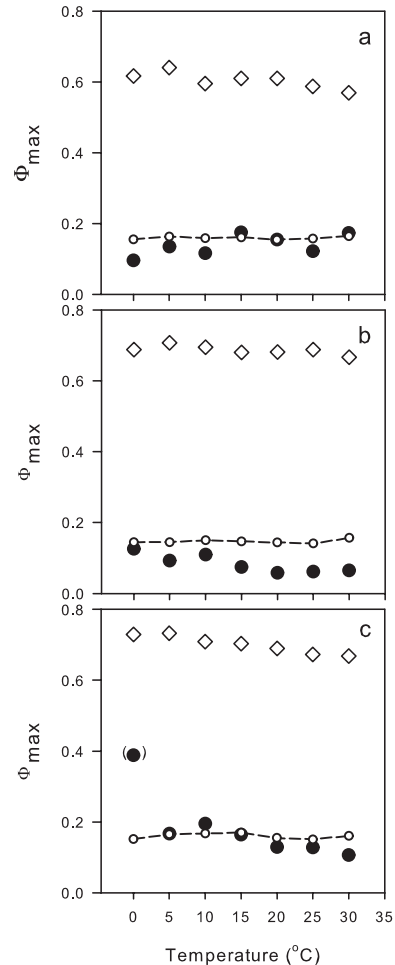
FIG. 4. Maximum quantum yield for O 2 ( \Phi_{\text{O}_2_{\max}}^{\text{PSII}} , filled circles) and PSII ( \Phi_{\text{PSII}_{\max}} , open diamonds) as a function of temperature for (a) Prorocentrum minimum , (b) Prymnesium parvum , and (c) Phaeodactylum tricornutum . \Phi_{\text{O}_2_{\max}}^{\text{PSII}} was calculated based on the light absorption in PSII ( \bar{a}_{\text{PSII}} ) as was the theoretical maximum quantum yield for O 2 production (small open circles), which was calculated for each temperature (eq. 10, details in text).
