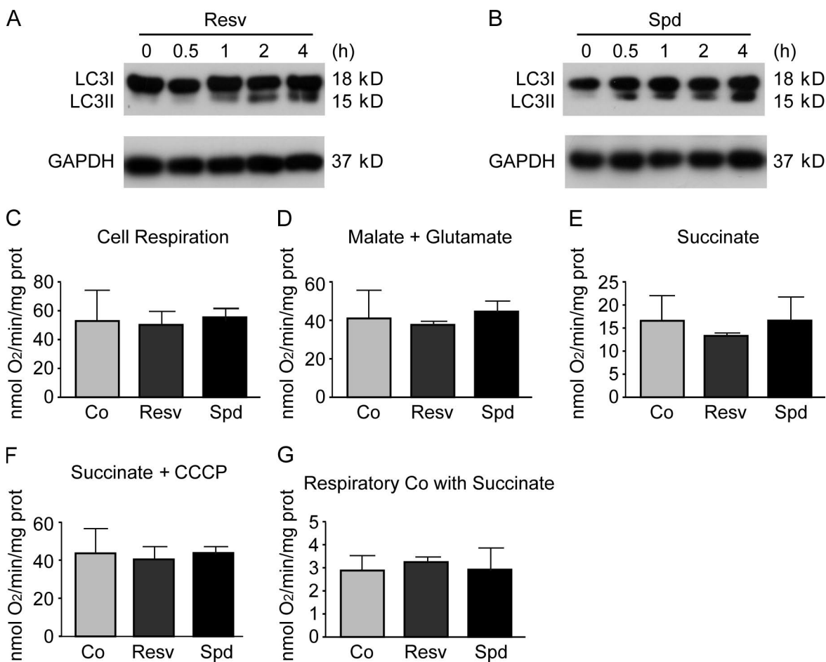
Figure S1. The kinetics of autophagy induction after 100- \mu M resveratrol and spermidine treatment and measurements of cell respiration and mitochondrial substrate oxidation in the absence (control) or presence of 100- \mu M resveratrol or spermidine. (A and B) Representative immunoblots showing endogenous LC3B lipidation in colon carcinoma HCT 116 cells treated with 100- \mu M spermidine (Spd) or resveratrol (Resv) for the indicated time. (C–G) HCT 116 cells were left untreated (Co, control) or treated with 100- \mu M resveratrol or spermidine for 4 h and then processed for the polarographic measurement of oxidative phosphorylation. Bars depict nanomoles of O 2 consumed per minute and milligrams of protein (prot; means \pm SD; n = 3 ). CCCP, carbonyl cyanide m -chlorophenyl hydrazine. GAPDH, glyceraldehyde 3-phosphate dehydrogenase.
