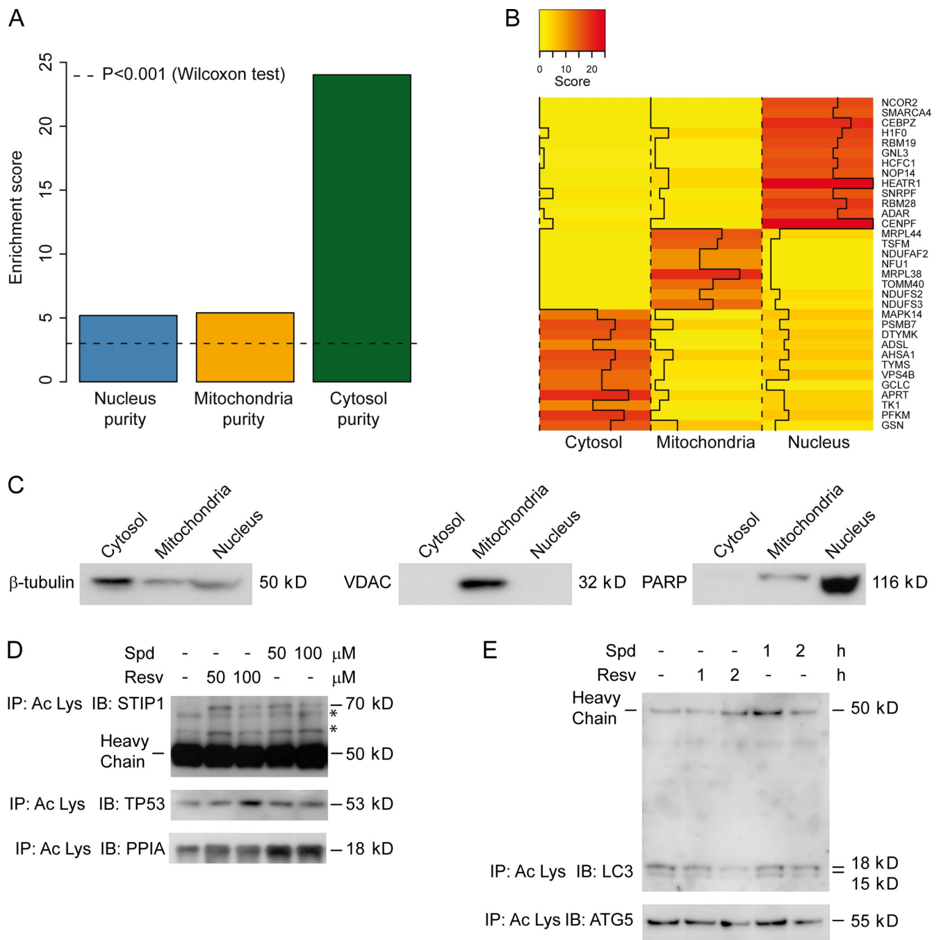
Figure S2. Measurement of SILAC fraction purity and analysis of the acetylation status of autophagy essential proteins after spermidine and/or resveratrol treatment. (A–C) Determination of the purity and quality of the organelle fractionation. (A) Fraction purity is measured by an enrichment score calculated from Wilcoxon testing for distribution location shift in compartment-specific peptides classified by GO cellular component terms compared with all identified peptides within the corresponding organelle fractions. The dashed line indicates a high significant score corresponding to P < 0.001 (Wilcoxon test). (B) Using a Western blot-like approach, 33 organelle-specific markers were selected and used to determine the purity of organelle fractions. The color key is a visualization of the fraction-specific number of identified peptides associated with the protein whose gene name is indicated as the row name. The fraction-wise relative number is indicated in the heat map trace histogram (black line). (C) Control immunoblots on the subcellular fractions used for the proteomic experiments. Cytoplasmic, mitochondrial, and nuclear fractions were blotted with antibodies specific for \beta -tubulin, voltage-dependent anion channel (VDAC), and histone H3. PARP, poly-(ADP-ribose) polymerase. (D–E) Human colon carcinoma HCT 116 cells were treated with resveratrol (Resv) or spermidine (Spd) at the indicated concentrations for up to 2 h, processed for immunoprecipitation (IP) with an anti-acetyl lysine (Ac-Lys) antibody, and then subjected to immunoblotting (IB) with the depicted antibodies. Asterisks represent nonspecific bands detected by the antibody.
