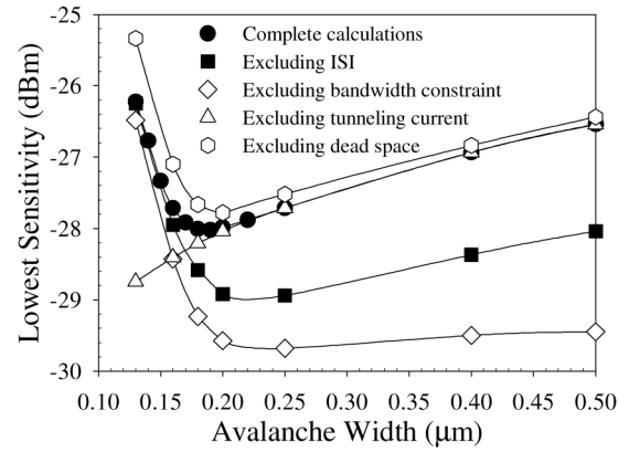
Fig. 4. Sensitivity versus avalanche width for the complete and various incomplete calculation conditions for a 10 Gb/s system. Different curves identify the distinct roles of ISI, device bandwidth, avalanche excess noise, and tunneling current.
