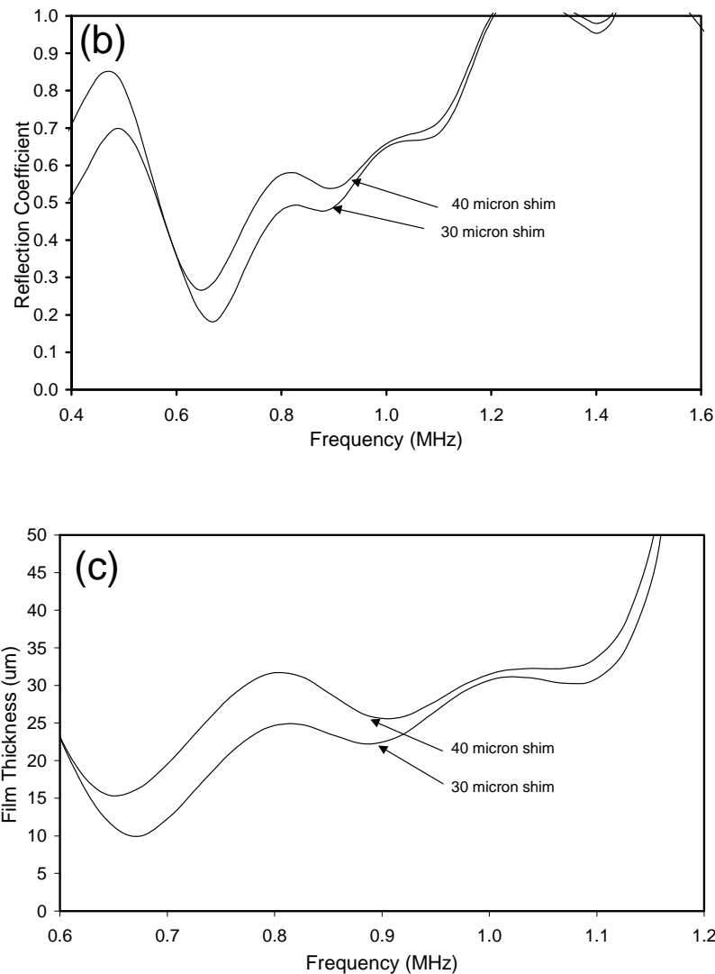
Figure 7. (a) Fourier transform of the pad surface reflection, (b) Reflection coefficient spectrum and (c) film thickness spectrum for 30 and 40μm oil films.
