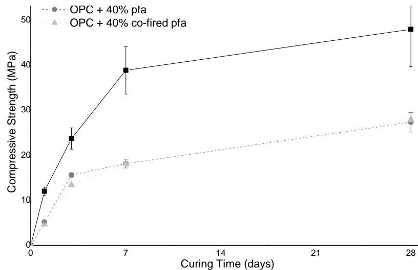
Figure 1: Compressive Strength Development of the Various Mixes.
