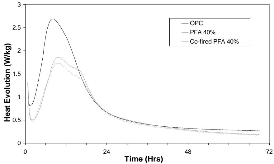
Figure 2: Isothermal Calorimetry Data for the Various Mixes
