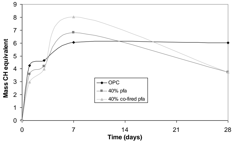
Figure 3: Amount of portlandite detected in the various pastes by TGA.
