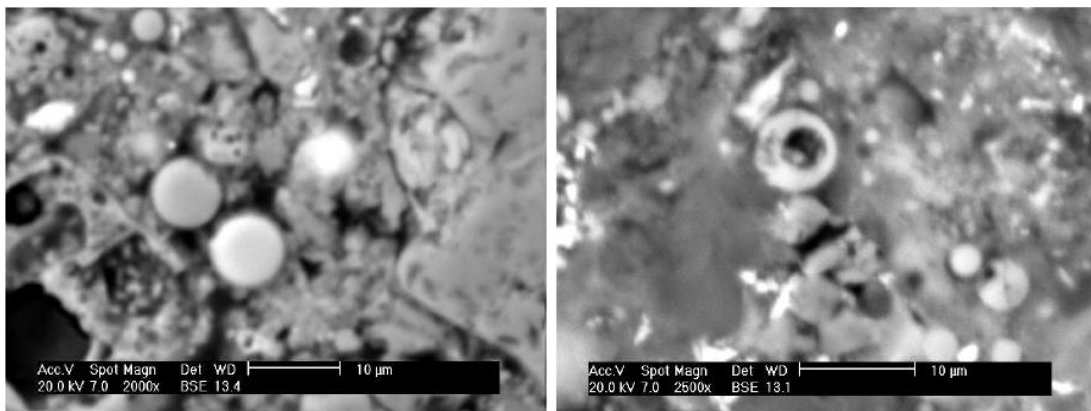
Figure 4: SEM Micrographs of the Blended Cement Mortars, (Co-fired pfa left, Conventional pfa right)
