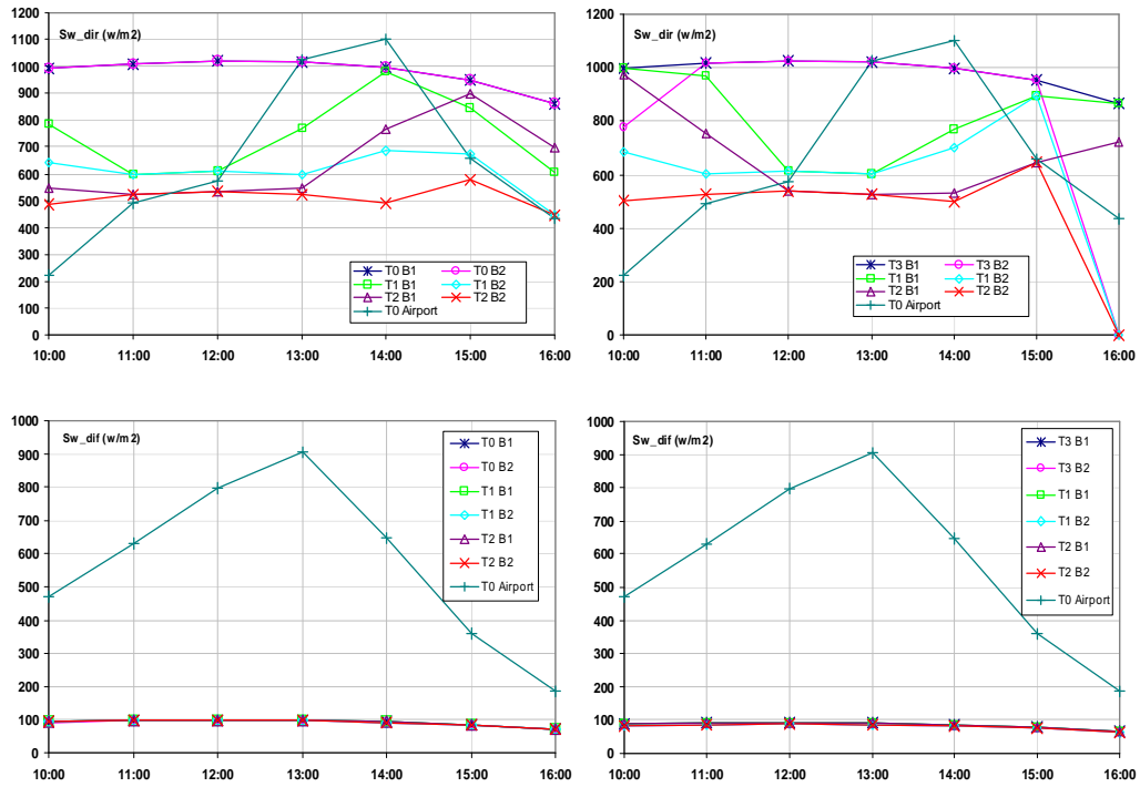
Fig.7/a, b, c, d: Sw.dir and Sw.dif at F1_B1 and F2_B2; left is C1 and right is C2.
