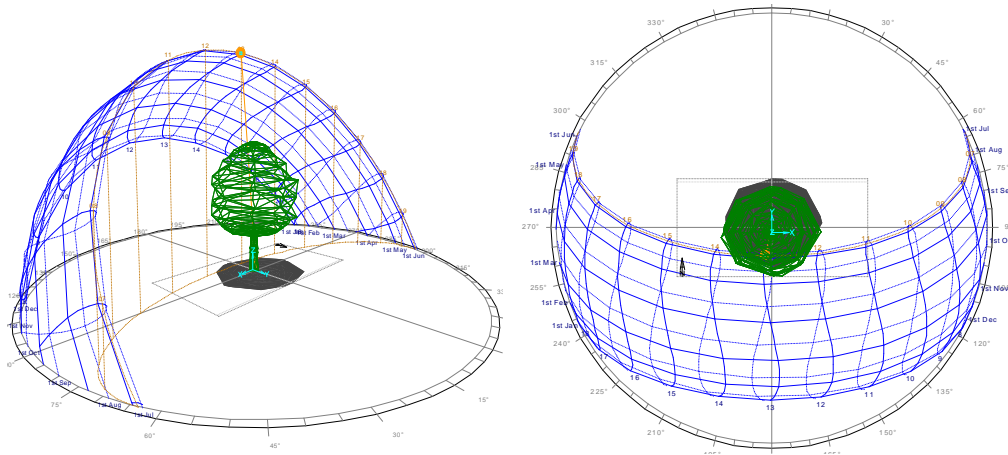
Fig.4: Schematic model by ECOTECT 5.6 for the Yellow Poinciana (following Shahidan et al., [36]) to indicate shadow of solar altitude of 82.40° on the simulated day, the 7 th of June at peak time of 13.00 LST, which is almost equal plantation ground area; i.e. the least LAI should be 1.
