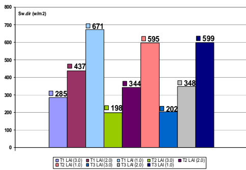
Fig.9/b. Short and long wave radiations recorded under trees upon different LAI values at 13.00 LST.
