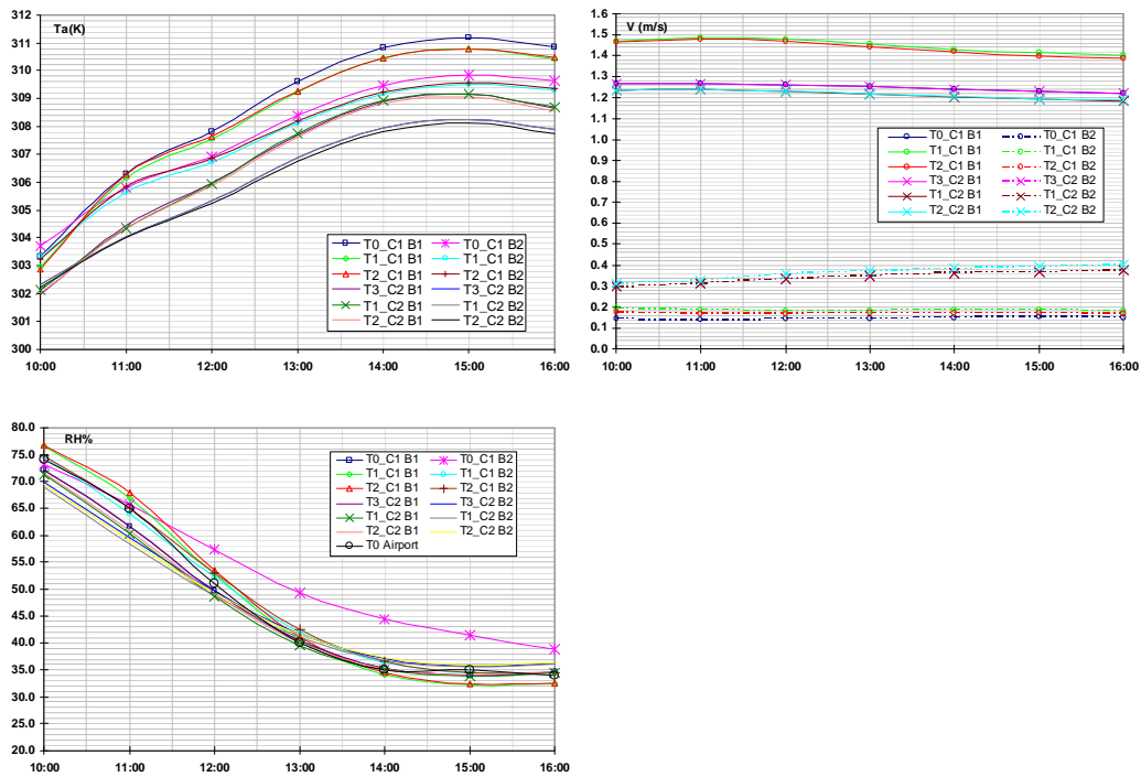
Fig.5: Comparison of Ta, V, and RH at F1_B1 and F2_B2 in both sites, respectively.
