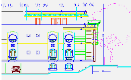
Fig.3: Side façade CAD illustration for the building-tree relation that could affect on the walls shadow, example is a design for the first author in C1.
