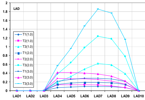
Fig.9/a: LAD values of T1, T2 and T3 upon 1, 2 and 3 LAI.
