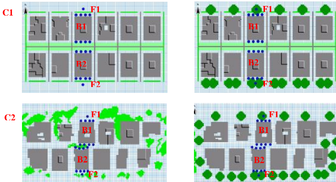
Fig.2/c, d, e, f: Illustration of sites before and after trees modifications with buildings and facades examined surrounded by snapshot receptor points; C1 is top and C2 is bottom.
