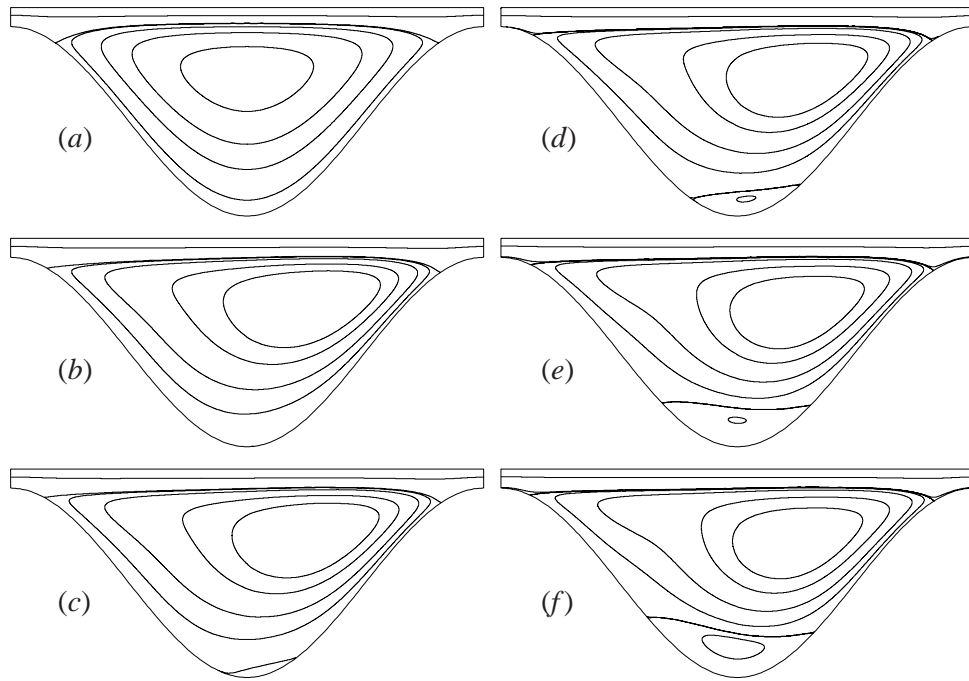
Figure 13: Streamline plots illustrating the generation and development of an inertially induced secondary eddy as Re increases: (a) Re = 0 ; (b) Re = 200 ; (c) Re = 260 ; (d) Re = 330 ; (e) Re = 450 ; (f) Re = 500 . The geometry is given by a = 2\pi/5 and h = 12\pi/25 , or, equivalently, H/A = 1.2 and \Lambda/A = 5 .
