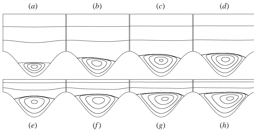
Figure 11: Effect of increasing inertia on eddy shape for H/A = 4 ( a-d ) and H/A = 2 ( e-h ), with the waviness of the lower plate a = 2\pi/5 \approx 1.257 . In ( a, e ) \text{Re} = 0 ; in ( b, f ) \text{Re} = 50 ; in ( c, g ) \text{Re} = 170 ; and in ( d, h ) \text{Re} = 300 .
