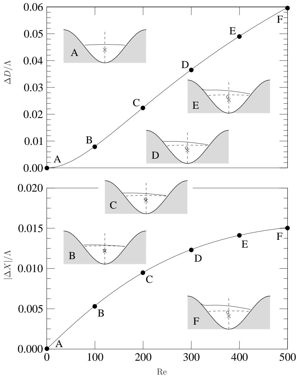
Figure 9: Effect of increasing inertia on the horizontal shift of the eddy centre, |\Delta X|/\Lambda (lower graph), and corresponding change in eddy depth, \Delta D/\Lambda (upper graph), for H/A = 14.2 and a = 2\pi/5 . The overlaid plots A to F show the separatrix and eddy centre position at the values of Re indicated by the corresponding black circles on the graphs. In plots B to F, the separatrix is shown as a solid line, and the eddy centre as an open circle. The Stokes flow separatrix and eddy centre position from A are included in each case as a dashed line and 'x' symbol, respectively.
