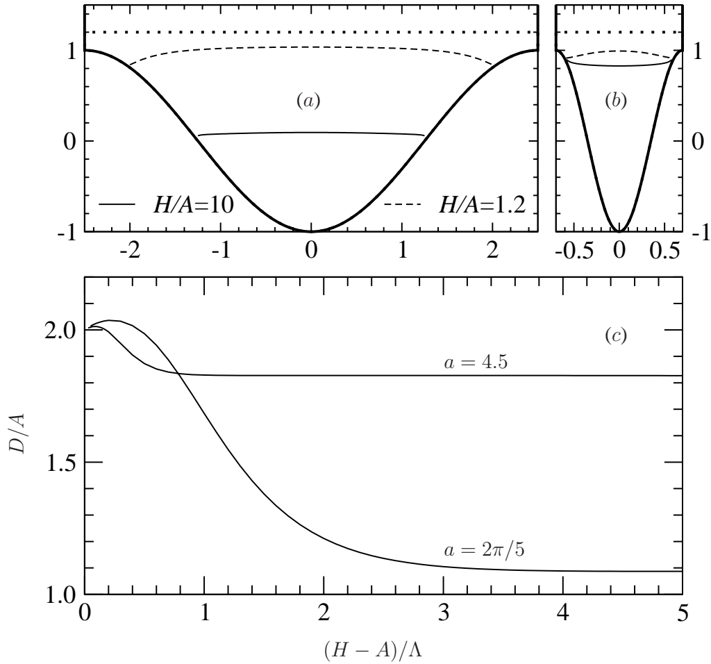
Figure 5: Comparison of the shape and position of the separatrix for different gaps and two different lower plate geometries. In (a) a = 2\pi/5 , and in (b) a = 4.5 . Lengths are scaled by A , and the dotted line in each plot shows the position of the upper boundary when H/A = 1.2 . Graph (c) gives the variation in eddy depth with the clearance.
