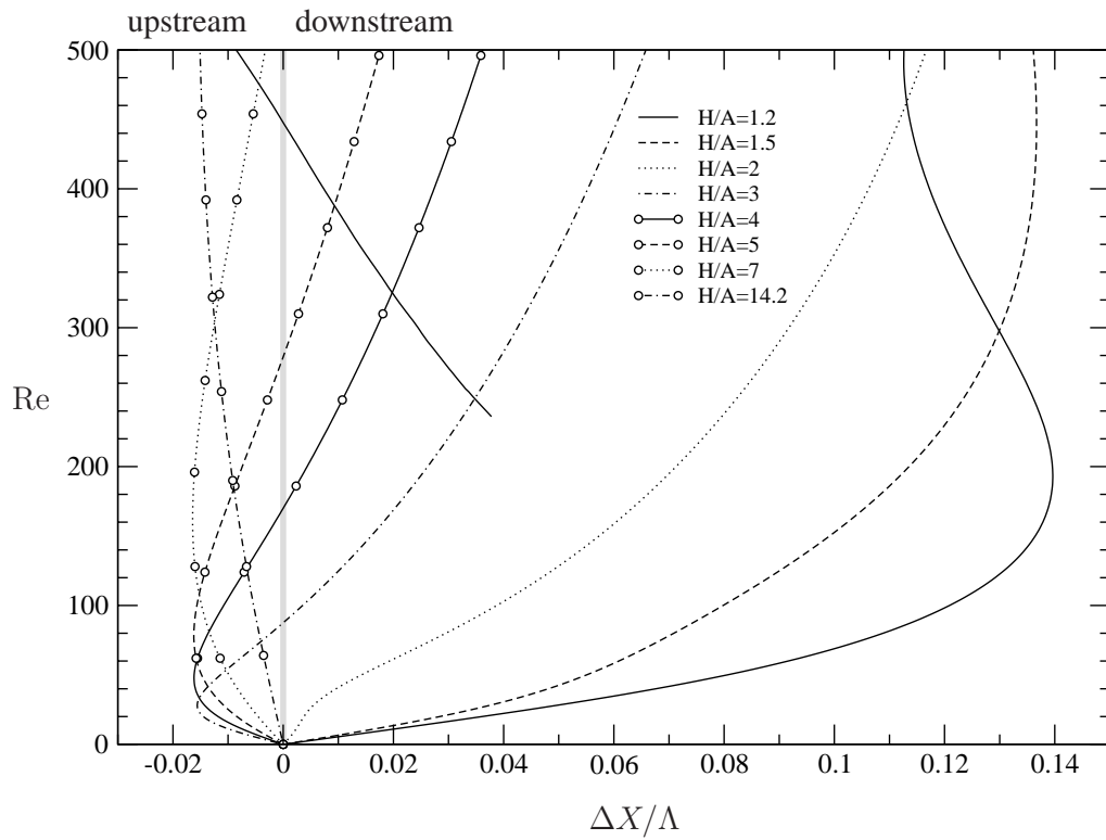
Figure 12: Effect of inertia on the horizontal shift of the eddy centre, \Delta X/\Lambda , for a = 2\pi/5 \approx 1.257 and a number of different gaps. The solid curve which begins near the centre of the plot corresponds to an inertially induced secondary eddy.
