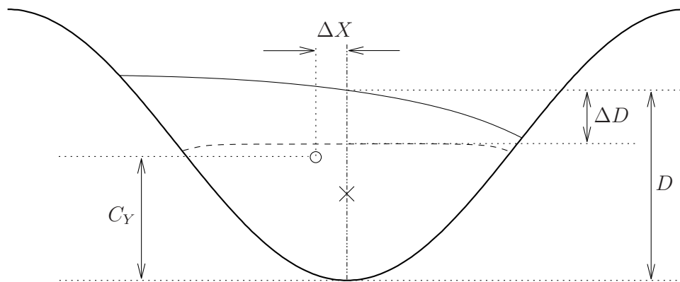
Figure 2: Sketch of the four measurables used to quantify resulting flow behaviour. The solid streamline and open circle mark the separatrix and eddy centre positions under general flow conditions, while the dashed streamline and cross give their corresponding positions for Stokes flow. The quantities \Delta X and \Delta D therefore refer to the difference in the position of the eddy centre and the eddy depth between the general and Stokes flow cases.
