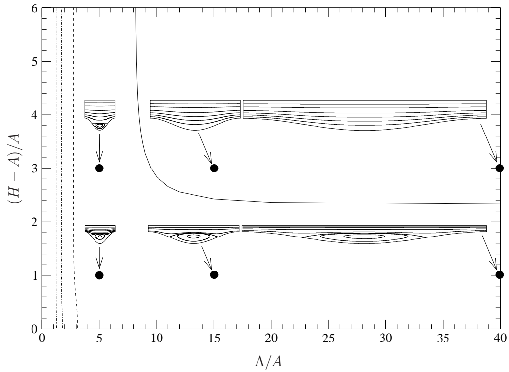
Figure 8: Critical curves of Fig. 6 replotted using the amplitude, A , of the lower plate as the length scale. The streamline plots show the flow structure for the parameter values at the indicated locations.
