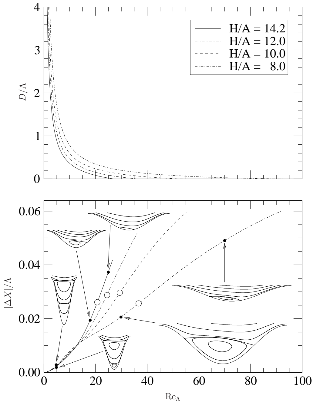
Figure 10: Effect of Re_\Lambda on the horizontal shift of the eddy centre, |\Delta X|/\Lambda , (lower graph) and on eddy depth, D/\Lambda , (upper graph) for large gaps and Re = 228 . The streamline plot inserts illustrate the flow structure for parameter values corresponding to the points shown as the black circles. The open circles mark the transition from a kinematically to inertially induced eddy.
