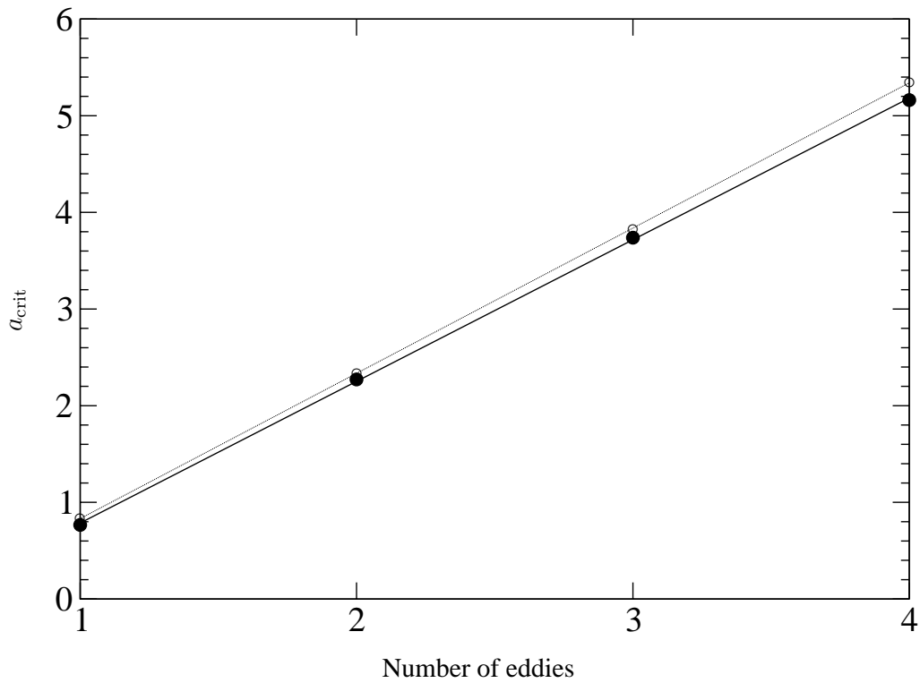
Figure 7: Critical values of waviness, a_{\text{crit}} , at which a new eddy appears. The solid circles represent critical values extracted from Fig. 6 at h - a = 10 . For comparison, the open circles indicate corresponding free-surface film results for a Nusselt film thickness h_0 = 10 . The solid lines are linear fits to the data.
