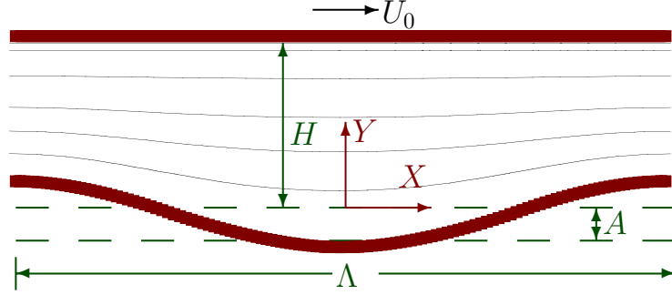
Figure 1: Schematic of the defining geometry for plane laminar shear flow between a flat moving upper and a fixed corrugated lower plate.
