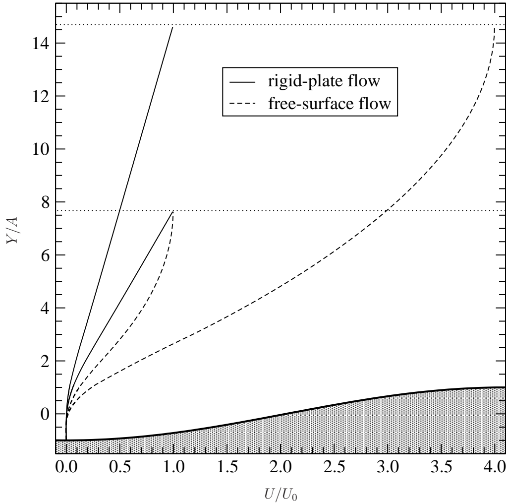
Figure 4: Velocity profiles along the vertical centreline. The curves illustrate the effect of doubling the mean gap (film thickness) on the velocity profiles in the case of rigid plate laminar shear (free-surface film) flow. Lengths are scaled by A . The thick solid line indicates the lower plate surface, and the dotted lines indicate the positions of the upper boundary when H_f/A = 7 ( H/A = 7.68 ) and H_f/A = 14 ( H/A = 14.698 ).
