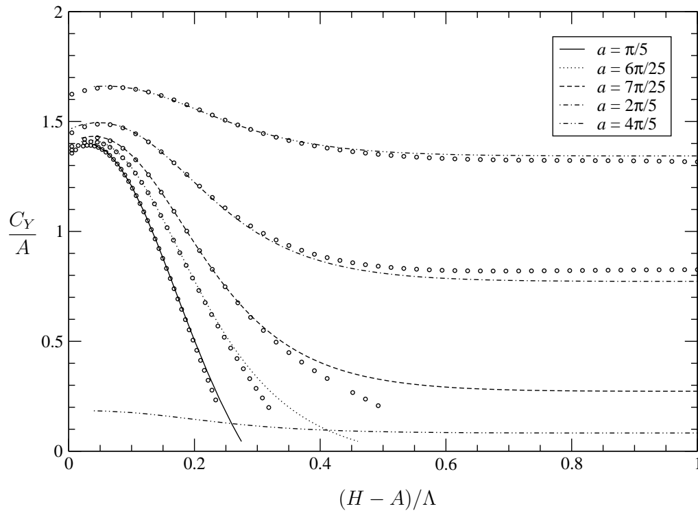
Figure 3: Calculations of the height, C_Y , of the eddy centre above the bottom of the topography, as a function of the gap under Stokes flow conditions. The discrete points give corresponding semi-analytical results with N = 4 .
