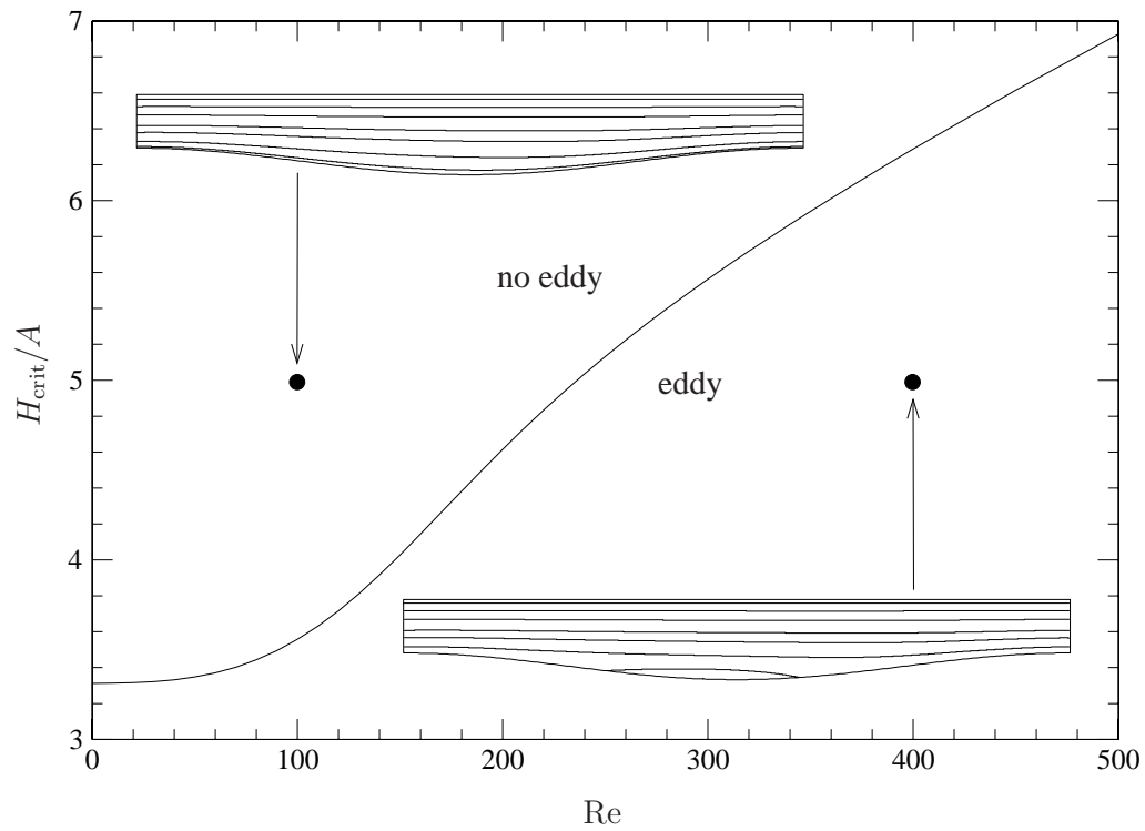
Figure 14: Effect of Reynolds number on the critical gap for the appearance of an eddy at long wavelengths. Here \Lambda/A = 50 , corresponding to a = \pi/25 \approx 0.1257 . The streamline plots correspond to the conditions at the indicated black circles.
