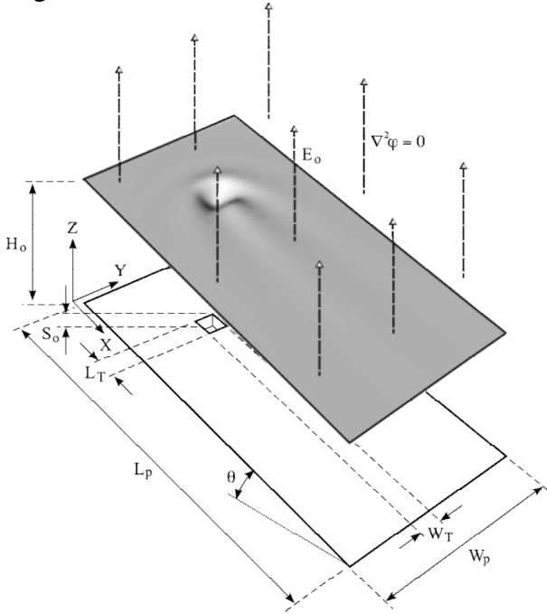
Fig 1: Gravity-driven flow over a trench topography in the presence of an electric field.
