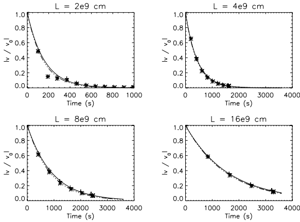
Fig. 5. As Fig. 3 for T_a = 2.0 MK.
