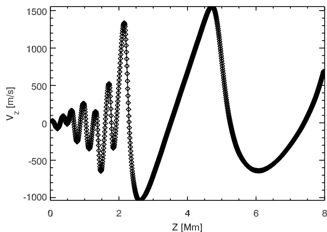
Fig. 8. Vertical velocity profile, taken at the centre of the simulation box, from the simulation of the wave conversion in the solar corona taken at t = 230 s. The conversion of linear waves into non-linear occurs at z = 2000 km.
