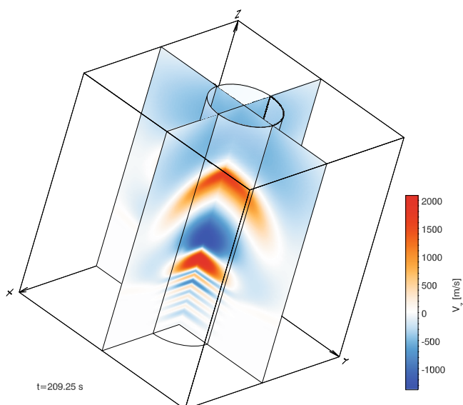
Fig. 9. Snapshot from the simulation of the wave propagation and conversion in magnetic solar chromosphere and corona taken at t = 209 s. The magnetic field, which is sketched by a cylinder in the figure, acts as a waveguide and suppresses the energy propagation outside the magnetic flux concentration.
